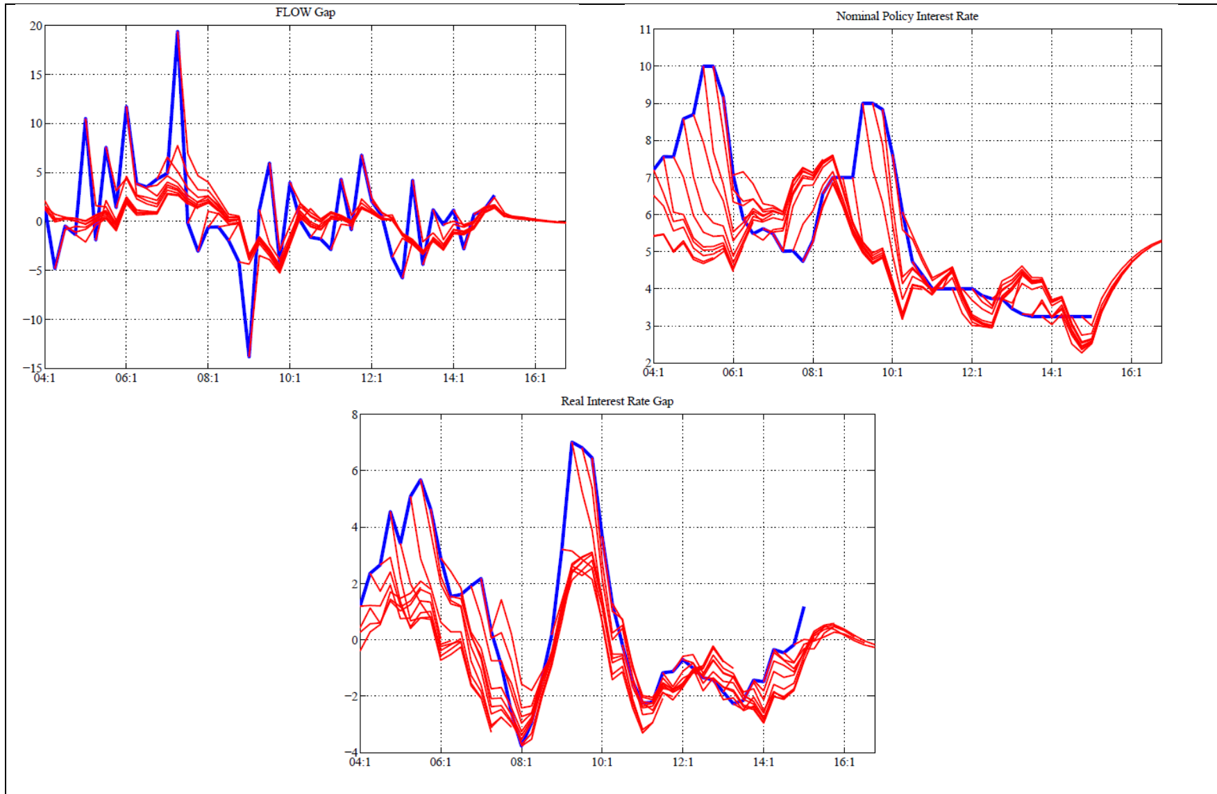
Figure 4. In-sample simulations
