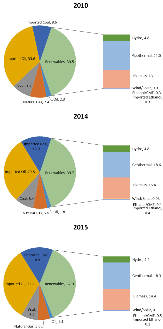
Figure 2: Philippines Primary Energy Mix, 2010, 2014-2015 (in percent)
