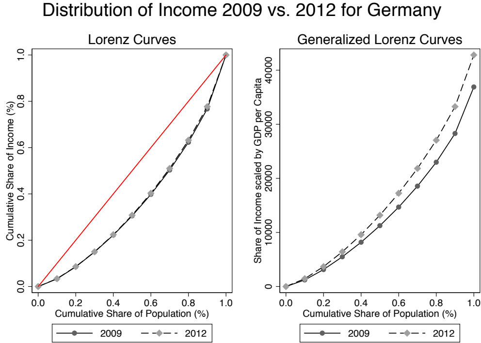
Figure 5: Lorenz and Generalized Lorenz Curves for Germany
