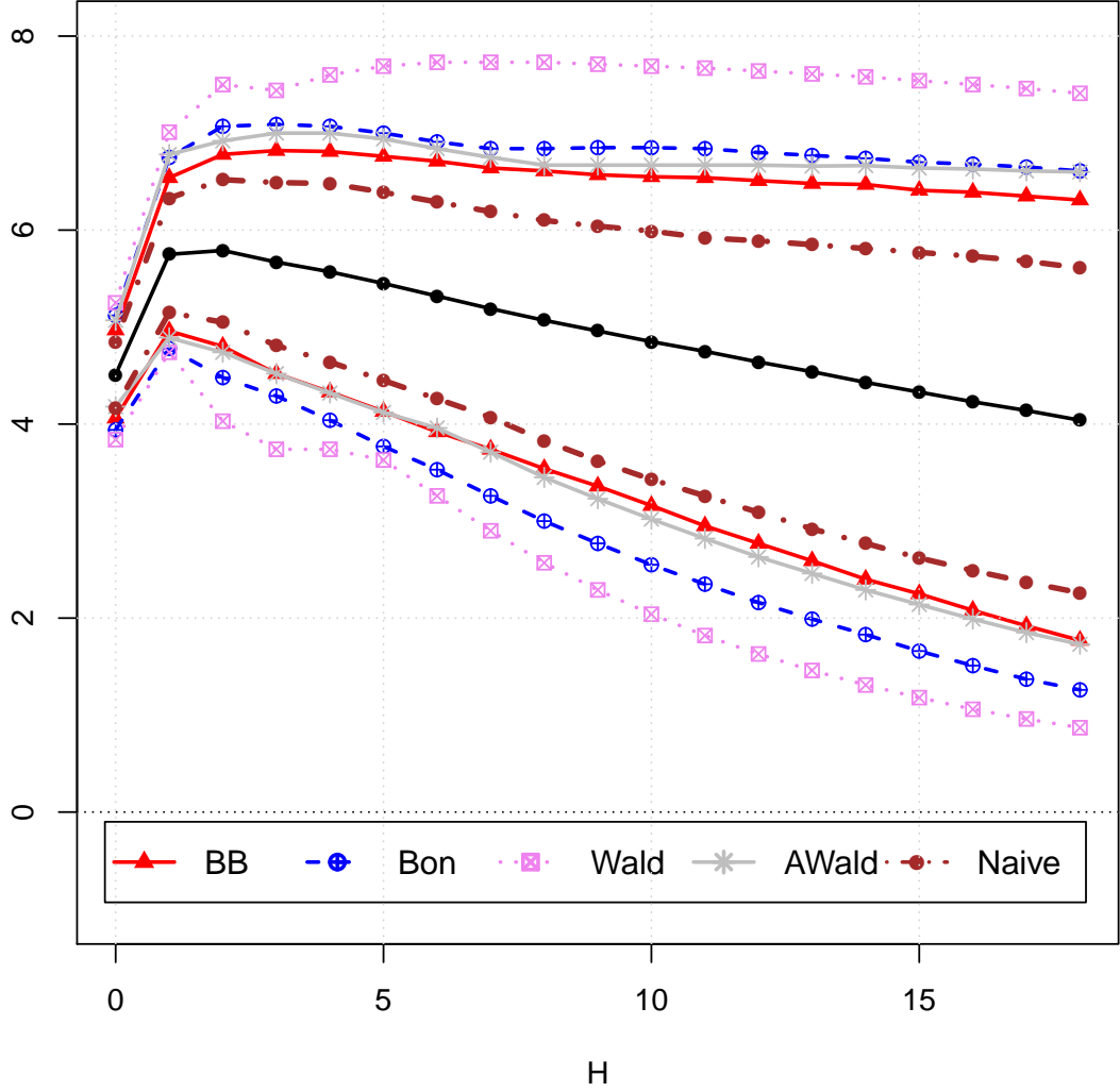
Figure N.8: Estimated impulse response of real_t to a one-standard-deviation shock in \varepsilon_{t,2} over a maximum propagation horizon of H = 18 (solid line with circles) and the corresponding nominal 90% joint confidence bands.
