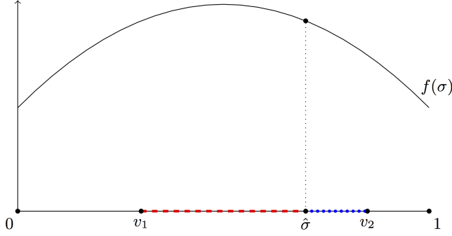
Figure 1: Illustration of an outcome given v_1 and v_2 where the ideal approach is \hat{\sigma} .
