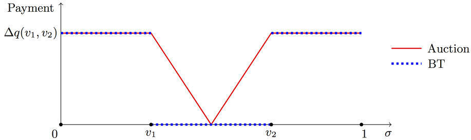
Figure 2: Comparison of payments in an auction and a bonus tournament.
