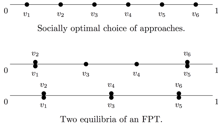
Figure 3: Equilibria when n = 6 .
