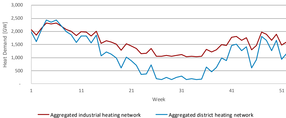
Figure 18: Weekly heat demand for the aggregated district heating network and the aggregated industrial heating network of Germany
