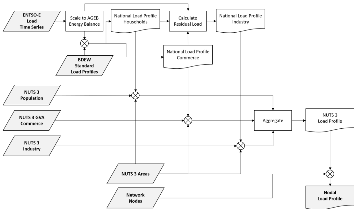
Figure 12: Calculation of nodal demand
