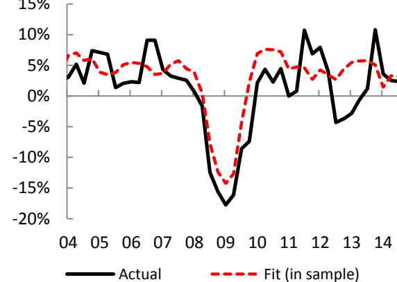
Chart A3: Japan - Fitted versus realized values
