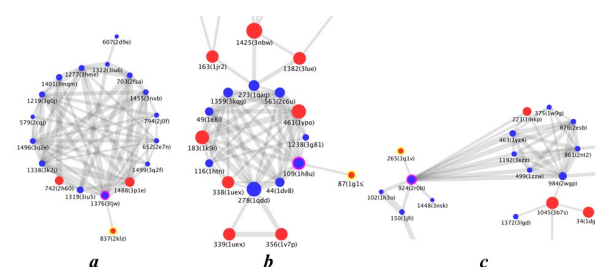
Figure 6. False negative predictions resulting from USA subnet maps. (a) A blue node with a purple border, 1376 is a hub node directly connected to USA number 837 (a red node with a yellow border), which is part of the protein 2klz, (b) The purple circle node 109 is a hub node directly connected to node 87 (PDB ID: 1g1s), (c) Node 265 belongs to the protein 1q1v and is connected to the hub node 924.
