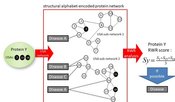
Figure 3. Illustration of the computation. First, protein Y is decomposed into three USAs. A local structural similarity is constructed using all USAs from all protein structures. Known diseases are mapped to USAs. RWR navigates the networks and generates a score for disease prediction for the given protein Y. Note that its score comes from the USAs 3, 15 and 18 that compose protein Y.
