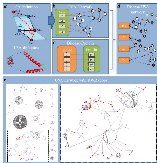
Figure 1. Research framework. (a) Encoding the Local Structure based on the SA definition. The USA is defined as extending the SA in a broader range and including the flexibility and stability of the secondary structure, (b) Assembling the USA complex network, in which nodes represent USAs and links represent structural similarity based on the results of all-against-all USA alignment, (c) Compiling the associations between diseases and proteins from the OMIM database, (d) Mapping both protein-USA and disease-protein relations, (e) The figure illustrates only a fragment of the USA complex network and the scores resulting from the RWR computation. Each node in the graph represents a USA, and the entire network is composed of 1511 nodes (USAs) and 3091 links (structural similarity relationships). The red and blue nodes represent disease-causing and non-disease-causing USAs, respectively. The size of each node represents its RWR score. A connection between two nodes means that the USAs have good structural similarity, and the width of the connection is related to the E-value of the USAs' structural similarity.
