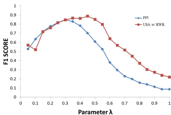
Figure 5. Prediction results of the F1-score graph. Prediction made at a threshold value \lambda of 0.45 were the most accurate, and the optimal F1-score was 0.8874. Networks constructed using traditional protein-protein interactions, after RWR verification, had an optimal F1-score of 0.8474, which was lower than that of our proposed method.
