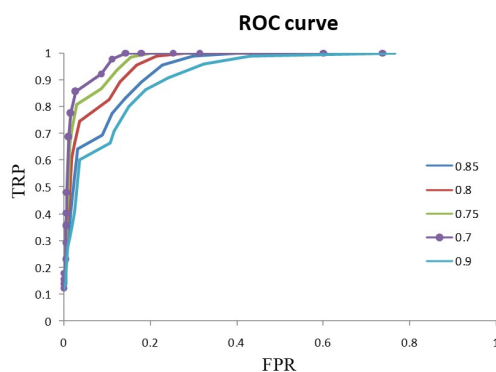
Figure 4. Optimal Parameter Analysis of the Restart Probability c .
