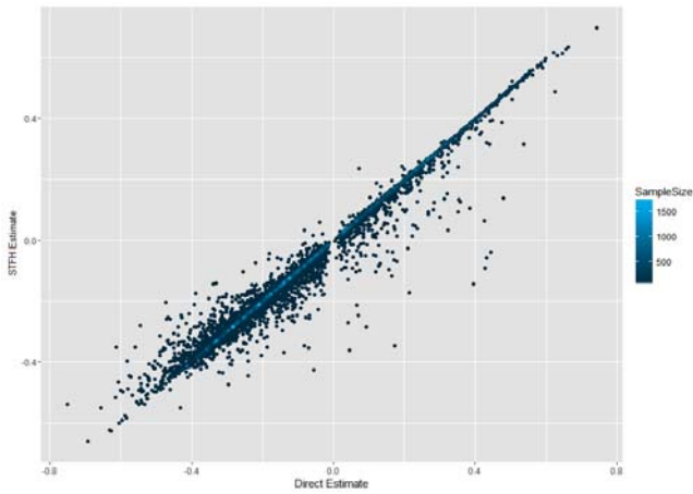
FIGURE 7 COMPARISON OF THE DIRECT ESTIMATES AND STFH ESTIMATES
