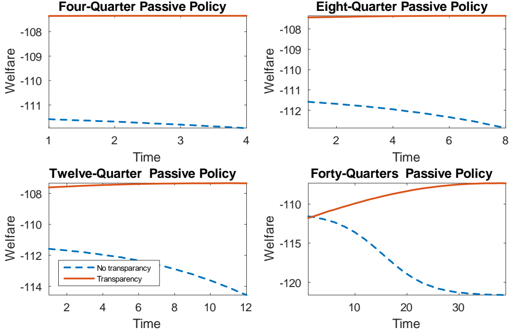
Figure 8: Evolution of welfare W_i(s_t(i)) defined in equation (6) as a passive policy of duration 4 (upper-left graph), 8 (upper right graph), 12 (lower left graph), and 40 quarters (lower right graph) is implemented under no transparency ( i = N ), the blue dashed line, and under transparency ( i = T ), the red solid line. Parameter values are set at the posterior mode.
