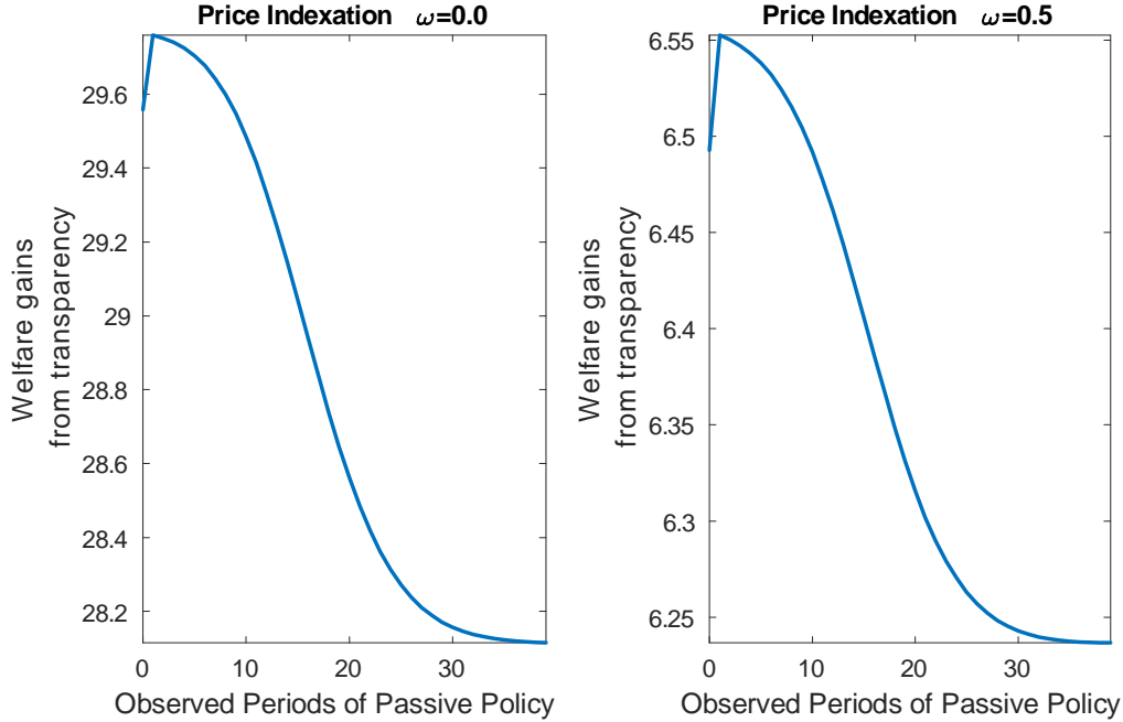
Figure 9: The graphs report the dynamics of the welfare gains from transparency as a function of the observed periods of passive policy ( \tau_t ) under no price indexation (left graph) and under partial price indexation, \omega = 0.5 , (right graph). The other parameter values are set at the posterior mode.
