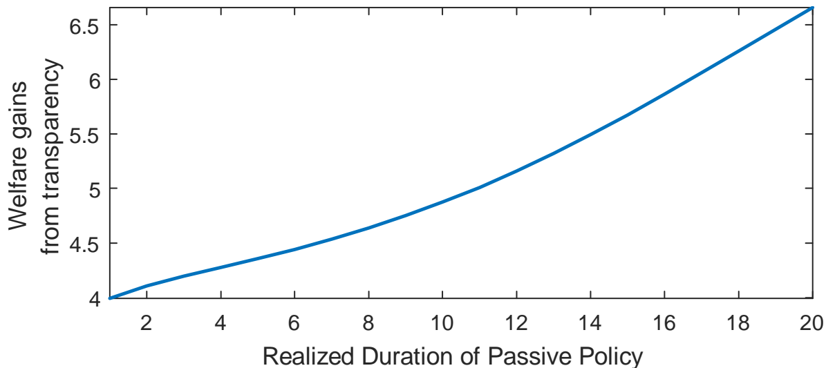
Figure 7: Average per-period welfare gains from transparency associated with passive policies of given realized durations. Parameter values are set at their posterior mode.
