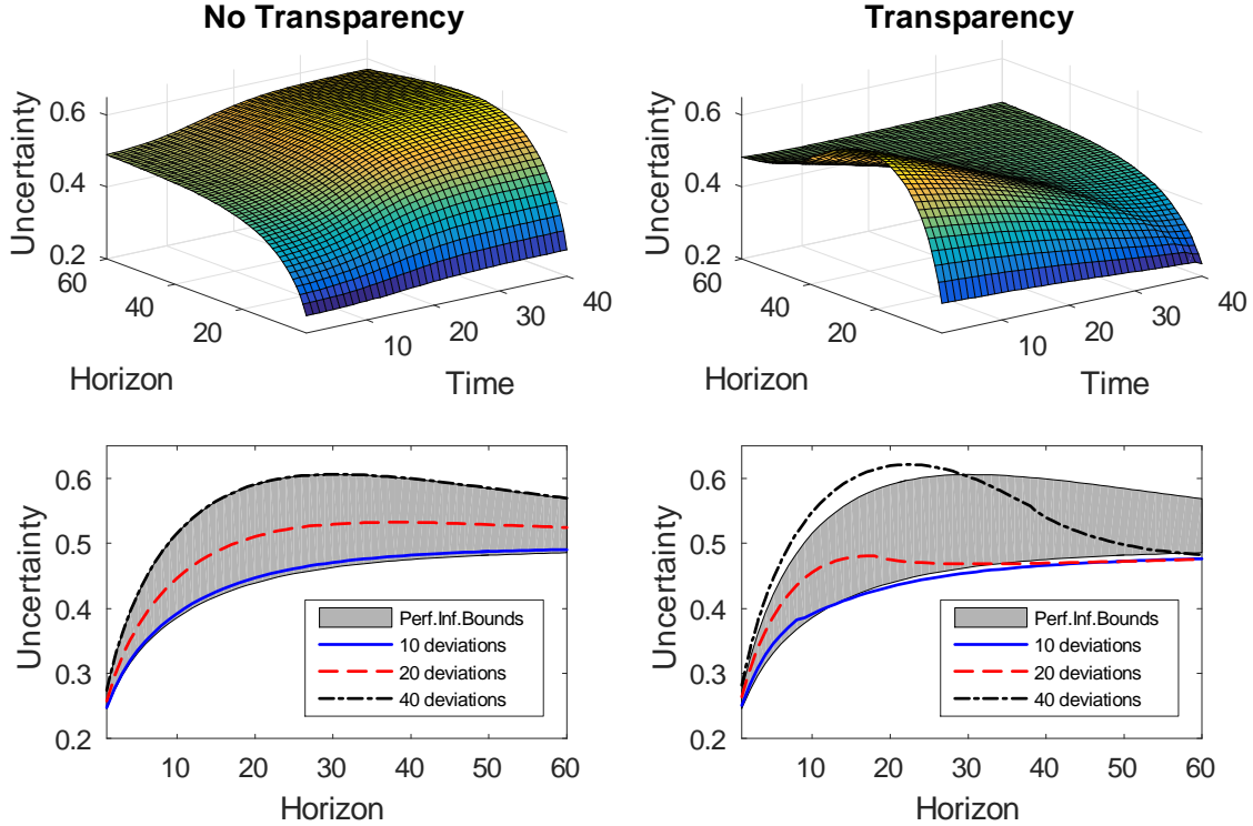
Figure 3: Upper graphs: Evolution of uncertainty about inflation at different horizons ( h ) over 40 periods of passive policy (time) under no transparency (left graph) and under transparency (right graph). The vertical axis reports the standard deviations in percentage points at the posterior mode. Lower graphs: Dynamics of uncertainty across horizons after having observed (left plot) or announced (right plot) 10, 20, and 40 consecutive quarters of passive policy. The gray areas denote the bounds for the dynamics of uncertainty about inflation across horizons when agents know the nature of the observed passive policy. The upper (lower) bound is when the passive policy is of the short-lasting (long-lasting) type. Parameter values are set at the posterior mode.
