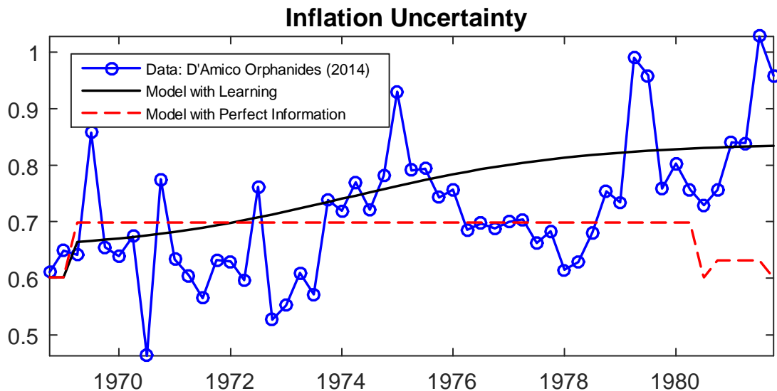
Figure 5: Long-Run Trend of Uncertainty about Future Inflation Predicted by the Model with Learning and the Perfect Information Model. The dynamics of inflation uncertainty resulting only from policy actions. The dynamics of uncertainty predicted by the two models is rescaled so that in 1968:Q4, inflation uncertainty is equal to the least square constant estimated using uncertainty in the data.
