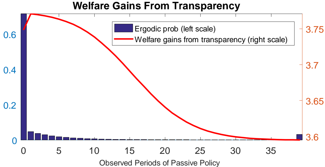
Figure 4: The solid line shows the dynamics of the welfare gains from transparency as a function of the observed periods of passive policy ( \tau_t ). The bars show the ergodic probability of observing the periods of passive policy on the x-axis ( \tau_t ). Parameter values are set at the posterior mode.
