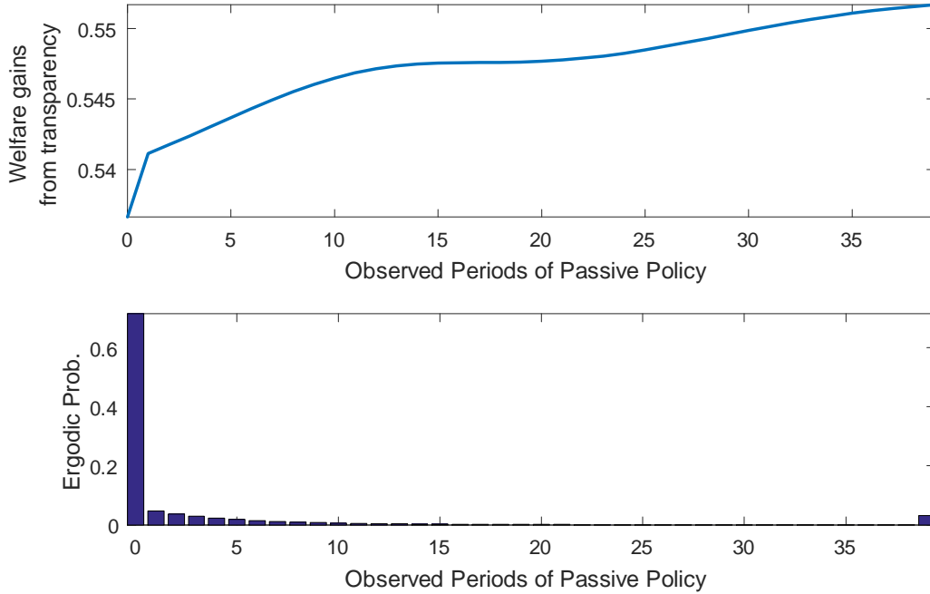
Figure 10: The upper graphs report the dynamics of the welfare gains from transparency as a function of the observed periods of passive policy ( \tau_t ) when the central bank is assumed to have limited information. The lower graph reports the ergodic probability of observing the periods of passive policy on the x-axis. Parameter values are set at their posterior mode.
