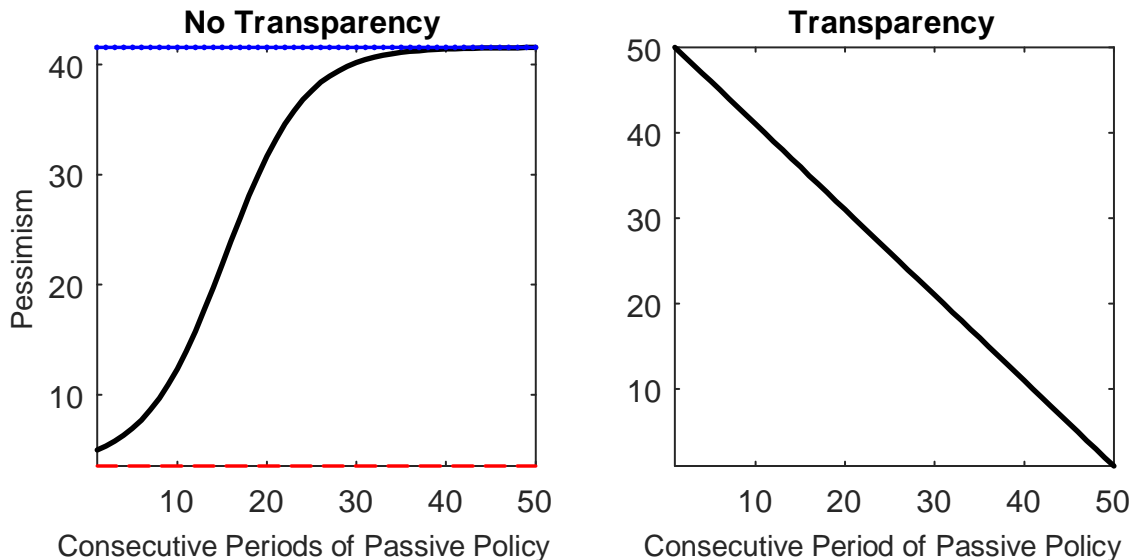
Figure 2: Pessimism on the vertical axis is measured as the expected number of consecutive deviations. On the left plot the two horizontal lines denote the smallest lower bound (1 - p_{22})^{-1} and upper bound of pessimism (1 - p_{33})^{-1} . These statistics are computed at the posterior mode.
