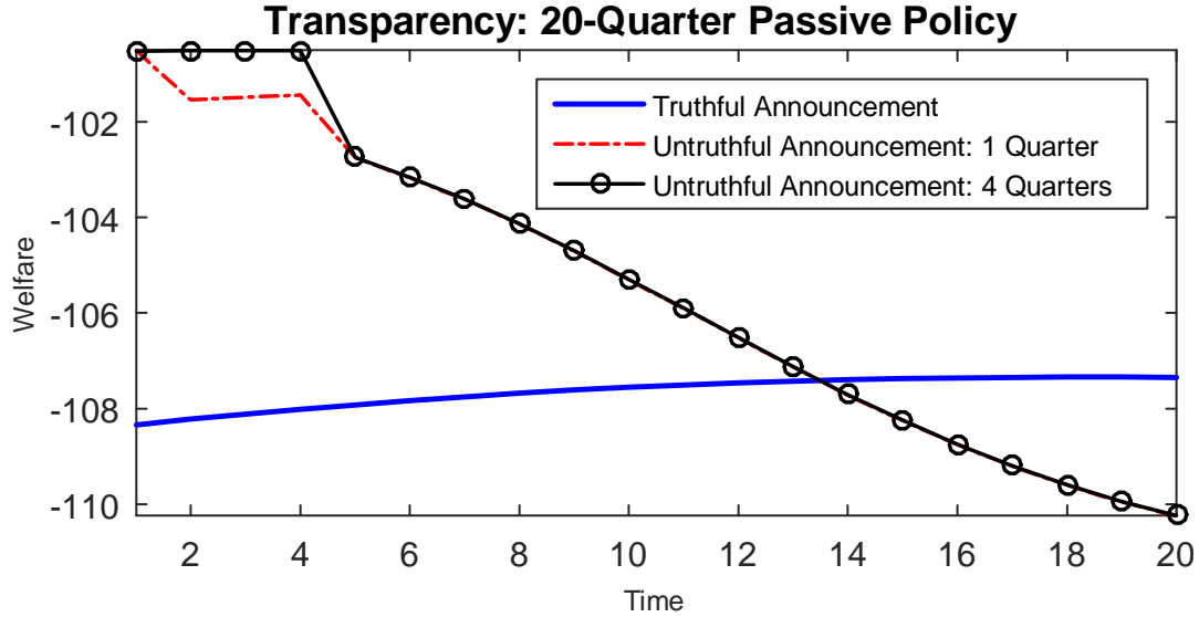
Figure 6: Welfare evolution as a 20-quarter deviation from the active policy is implemented under imperfectly credible announcements.
