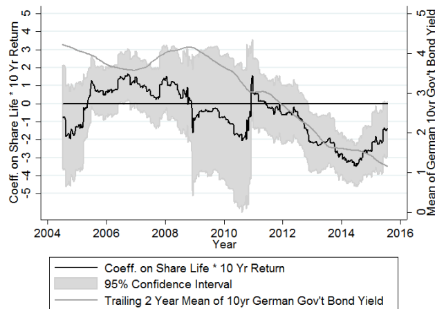
Figure 4: Estimates of Interest Rate Sensitivity for Continental European Insurers
