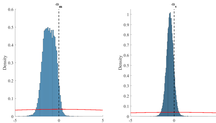
Figure 4: Prior (red line) and histogram of posterior distribution of regime switching reform parameters \alpha_m and \alpha_v . Source: Own calculation.
