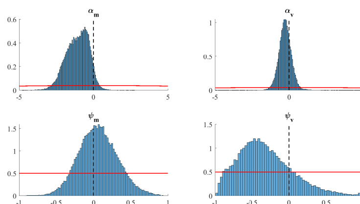
Figure 6: Prior (red line) and histogram of posterior distribution of regime switching reform parameters \alpha_m and \alpha_v and trend-cycle correlations \psi_m and \psi_v . Source: Own calculations.
