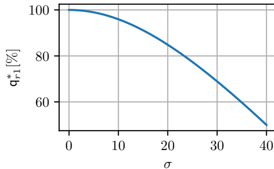
Figure 2: Impact on an increasing uncertainty via \sigma on the optimal first stage renewable bid q_{r,1}^* relative to the expected outcome \mathbb{E}[q_{r,1}] . The parameter to derive the figure were the aforementioned equations with D = 70 , \mu = 40 , a = 0.01 , b = 0 .
