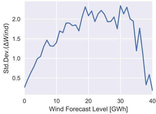
(c) Standard deviation of wind production clustered as to wind forecast level (1 GWh each)
