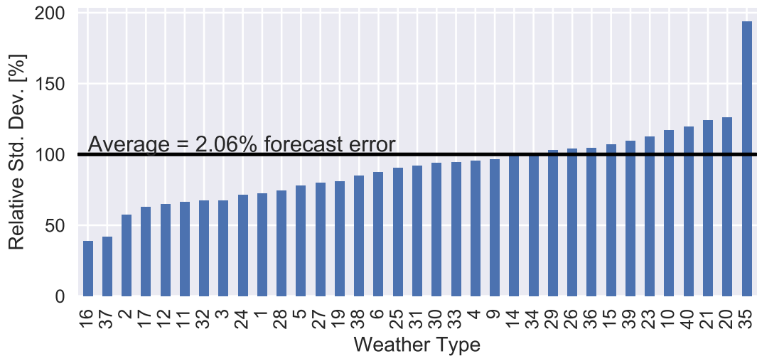
Figure 5: Relative standard deviations of the wind and solar forecast errors per weather type. The wind and solar forecasts errors are normalized by the monthly capacity. The standard deviation per weather class is relative to the standard deviation over all data (which is a forecast error of 2.06 %). Data covers July 2015 to December 2016.
