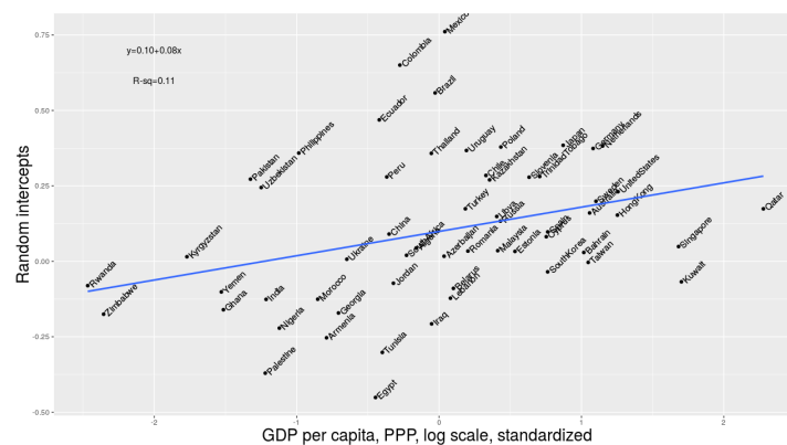
Figure 2: Random intercepts and GDP per capita
