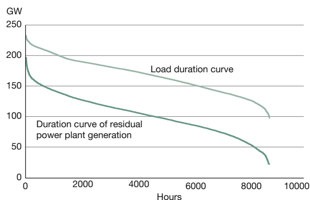
Figure 6 Load duration curve and duration curve of residual power plant park generation, PLEF region, 2030
