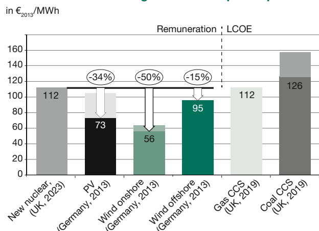
Figure 3 Average remuneration for new nuclear, PV and wind and LCOE for coal and gas-fired CCS power plants
