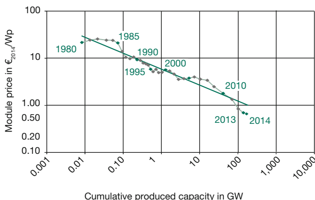
Figure 1 Historical price curve of PV modules, 1980-2014
