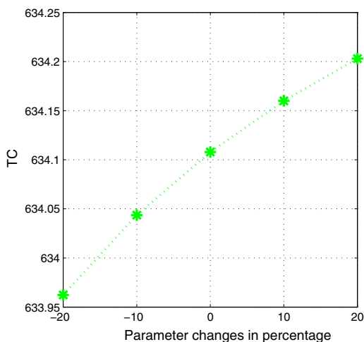
Fig. 8 Sensitivity on rework process rate in case 1
