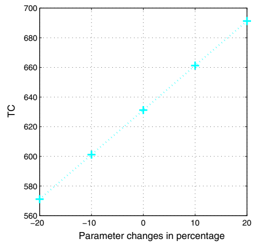
Fig. 15 Sensitivity serviceable holding cost in case 2
