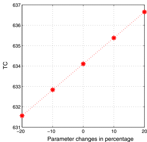
Fig. 7 Sensitivity on rework setup cost in case 1
