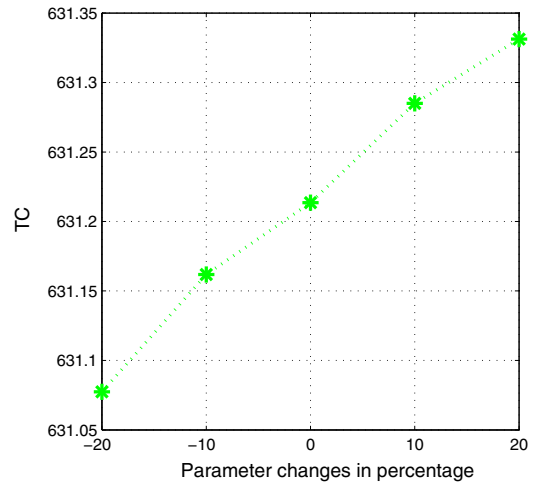
Fig. 14 Sensitivity on rework process rate in case 2
