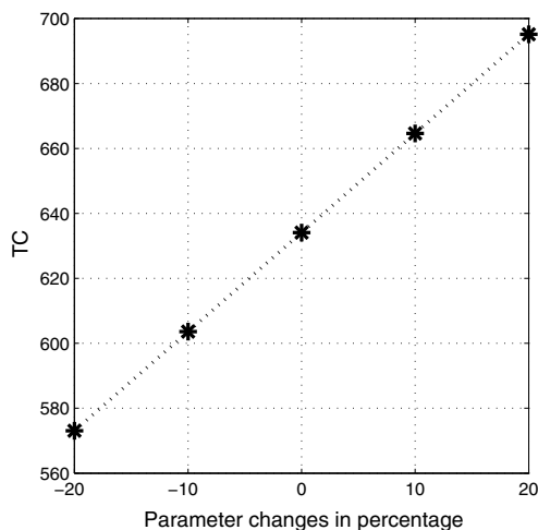
Fig. 6 Sensitivity on production setup cost in case 1
