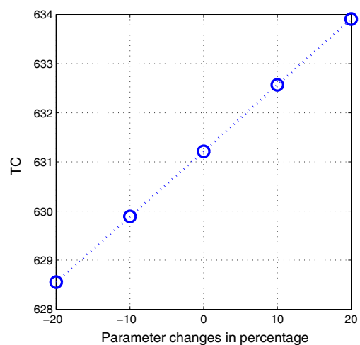
Fig. 16 Sensitivity on recoverable holding cost in case 2
