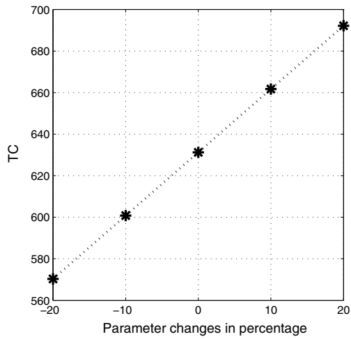
Fig. 12 Sensitivity on production setup cost in case 2
