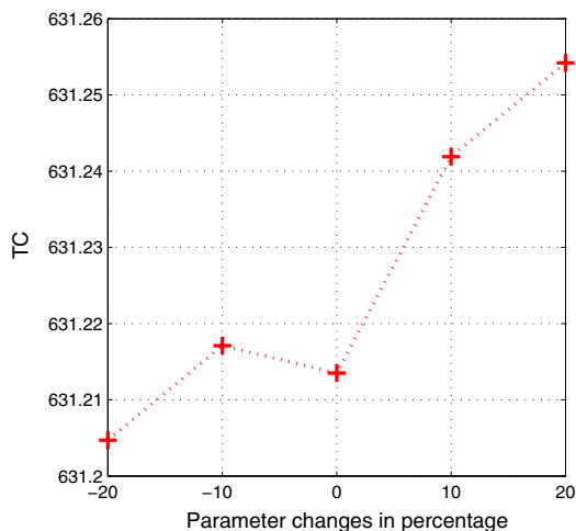
Fig. 17 Sensitivity on deteriorating cost in case 2
