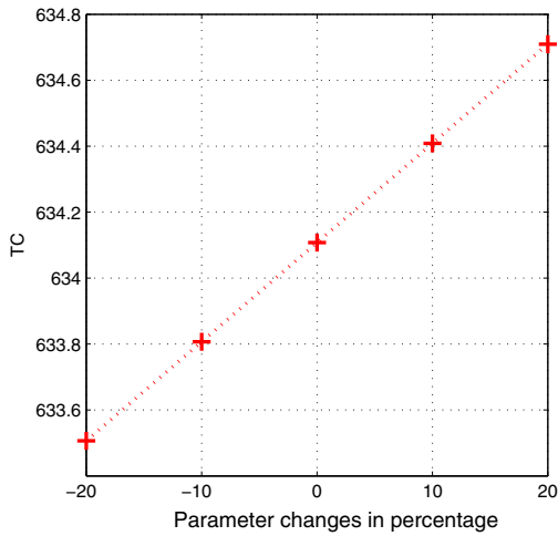
Fig. 11 Sensitivity on deteriorating cost in case 1
