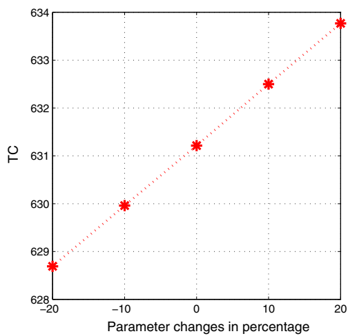
Fig. 13 Sensitivity on rework setup cost in case 2
