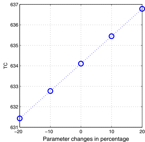
Fig. 10 Sensitivity on recoverable holding cost in case 1
