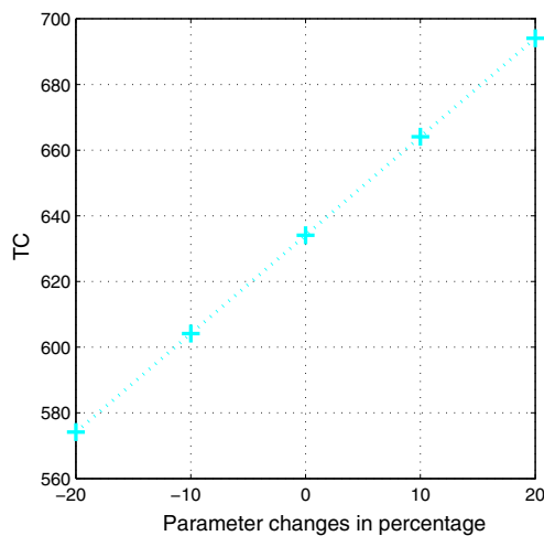
Fig. 9 Sensitivity serviceable holding cost in case 1
