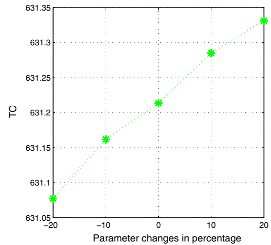
Fig. 14 Sensitivity on rework process rate in case 2
