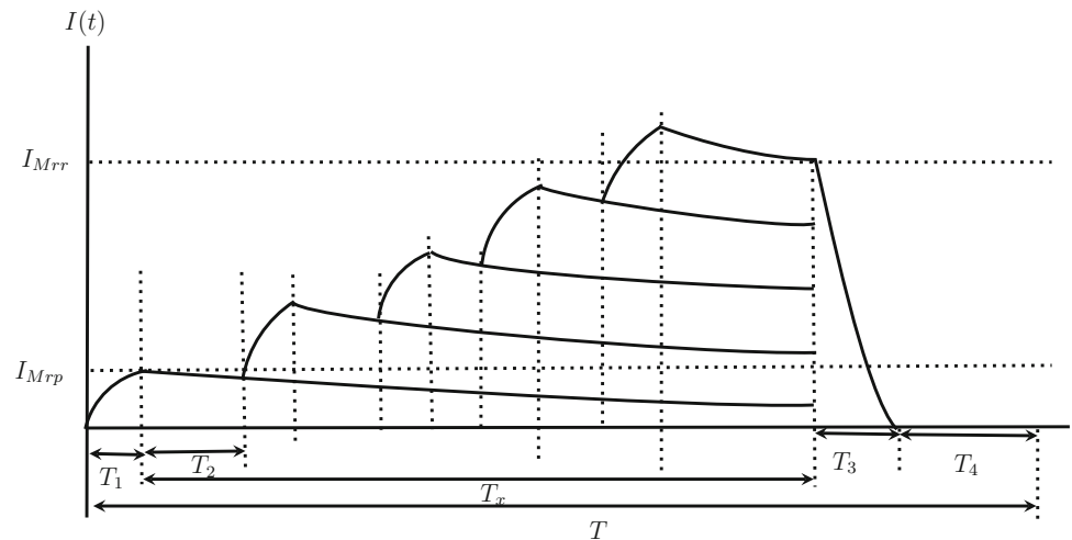
Fig. 3 Recoverable inventory level of five production setups and one rework
