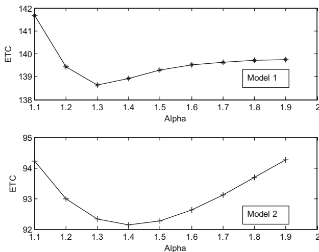
Fig. 1 ETC versus \alpha . S = 20 ; s = 5 ; \lambda = 1.5 ; \gamma = 0.8 ; N = 25 ; \theta = 1.5 ; \beta = 2 ; \delta = 0.7 ; \mu = 3 ; C = 20 ; c_1 = 1 ; c_2 = 1 ; c_3 = 28 ; c_4 = 3.6 ; c_5 = 50 ; c_6 = 50 ; c_7 = 1.01 ; c_8 = 1
