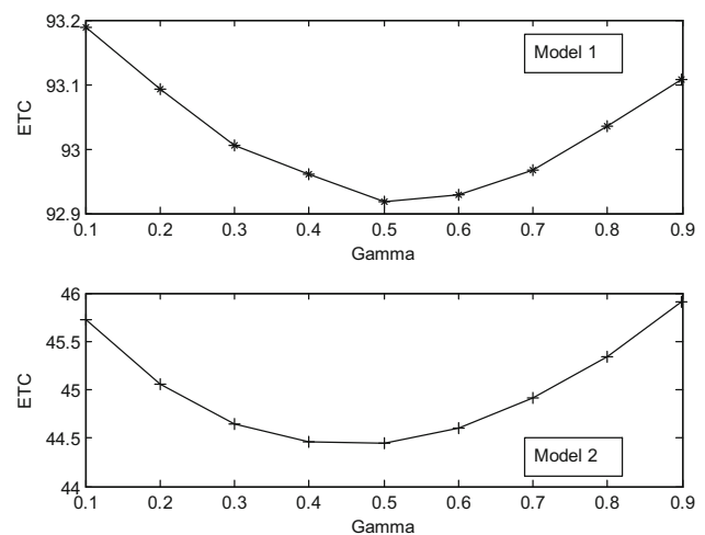
Fig. 3 ETC versus \gamma . S = 20 ; s = 5 ; \lambda = 1.5 ; N = 25 ; \theta = 1.5 ; \beta = 2 ; \delta = 0.7 ; \mu = 3 ; \alpha = 1.5 ; C = 20 ; c_1 = 14 ; c_2 = 1 ; c_3 = 3 ; c_4 = 3 ; c_5 = 3.3 ; c_6 = 6 ; c_7 = 4 ; c_8 = 1
