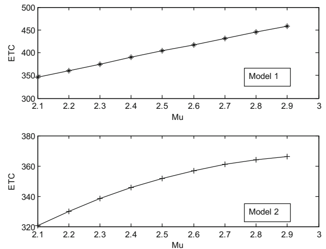
Fig. 2 ETC versus \mu . S = 20 ; s = 5 ; \lambda = 1.5 ; \gamma = 0.8 ; N = 25 ; \theta = 1.5 ; \beta = 2 ; \delta = 0.7 ; \alpha = 1.5 ; C = 20 ; c_1 = 1 ; c_2 = 1 ; c_3 = 1 ; c_4 = 1 ; c_5 = 1 ; c_6 = 1 ; c_7 = 150 ; c_8 = 1
