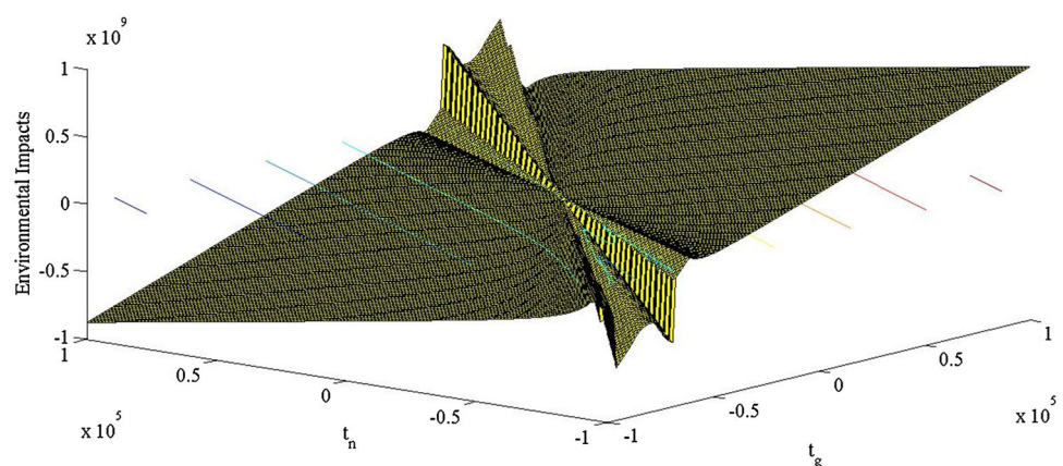
Fig. 1 Surface of objective function in first scenario (EIs)
