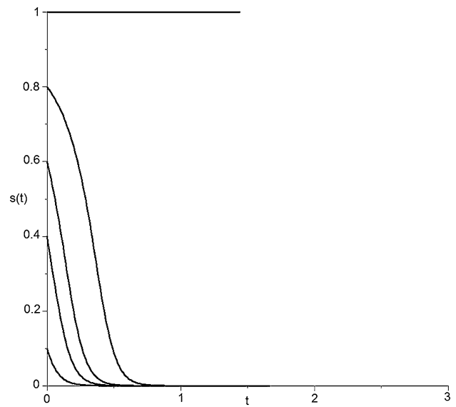
Fig. 6 Trajectories of ds/dt in second scenario
