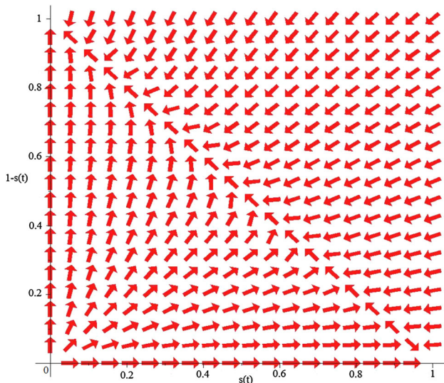
Fig. 3 Convergence to ESS (1, 0) or (0, 1) in first scenario
