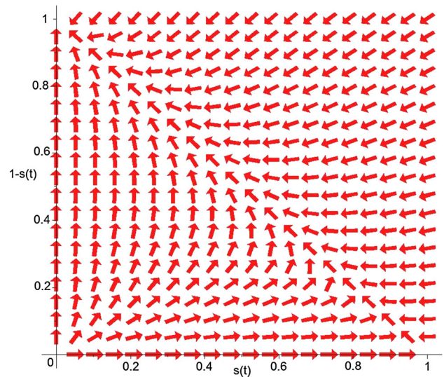
Fig. 5 Convergence to ESS (1, 0) or (0, 1) in second scenario
