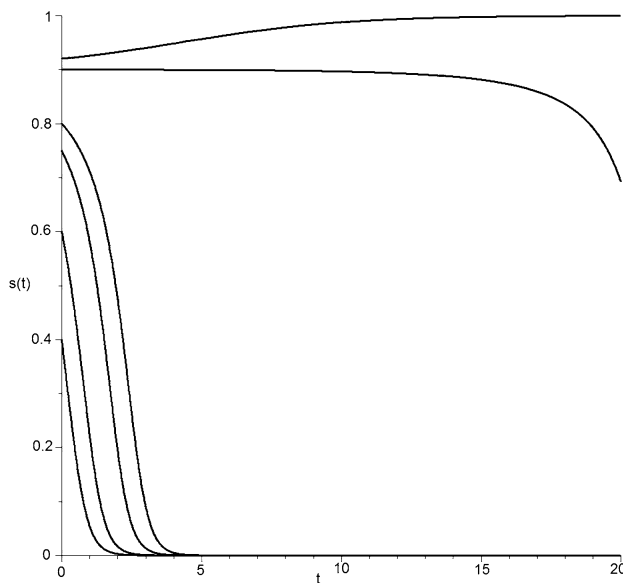
Fig. 4 Trajectories of ds/dt in first scenario
