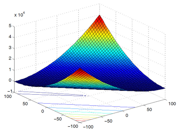
Fig. 10 The rotated hyper-ellipsoid function
