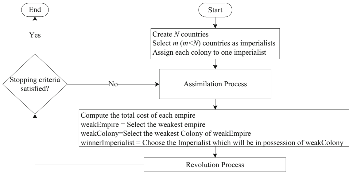
Fig. 2 Flowchart of ICA
