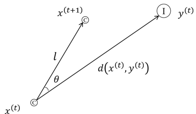
Fig. 1 Movement of a colony toward its imperialist during the assimilation process
