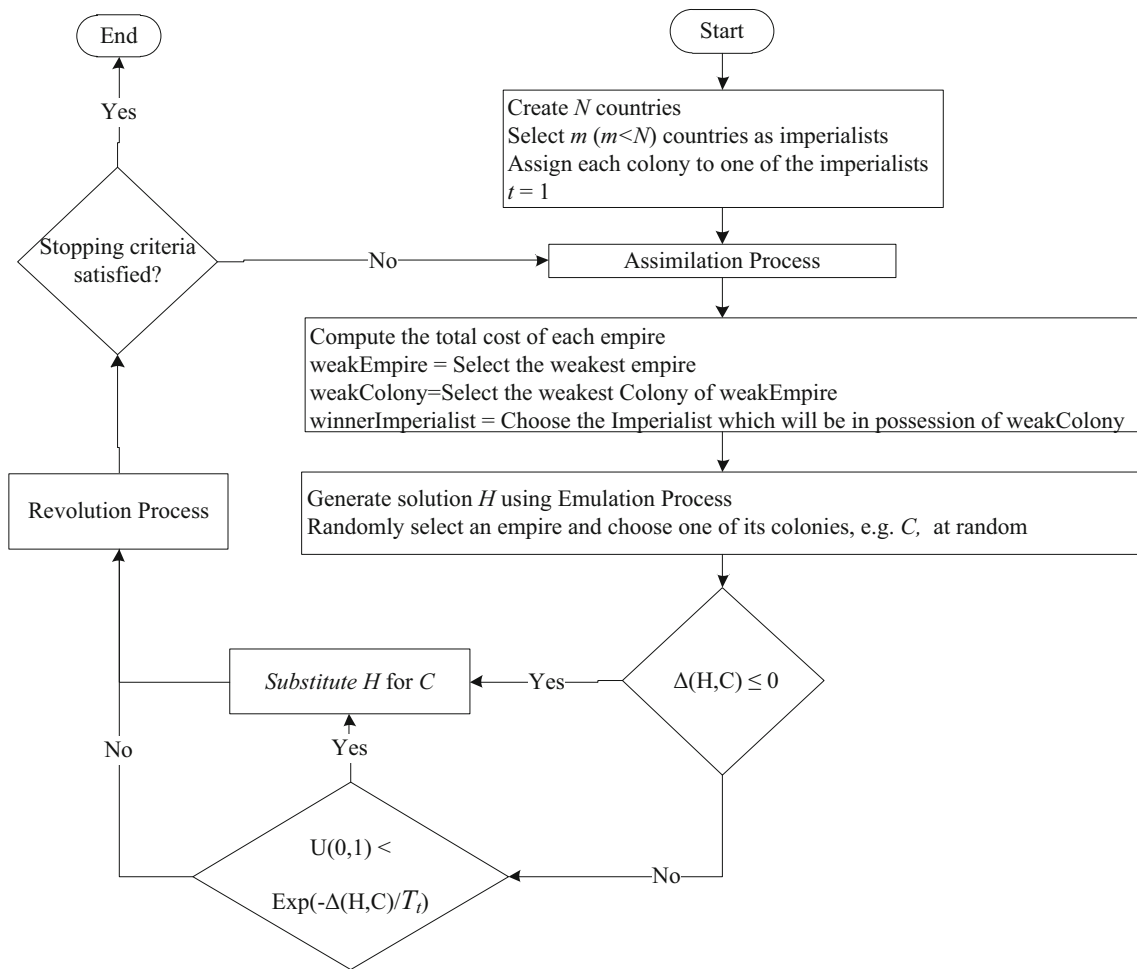
Fig. 5 Flowchart of the proposed hybrid algorithm
