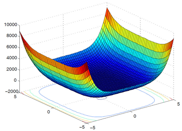
Fig. 14 The six-hump camel-back function
