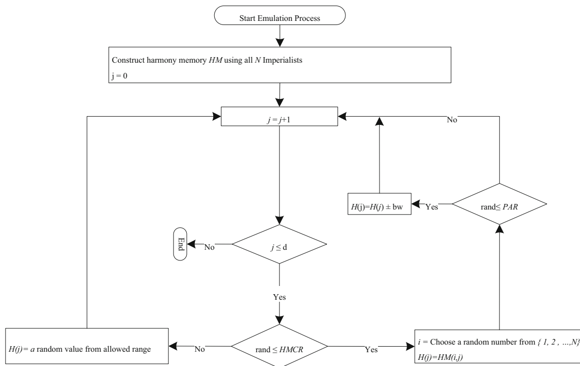
Fig. 4 The emulation process
