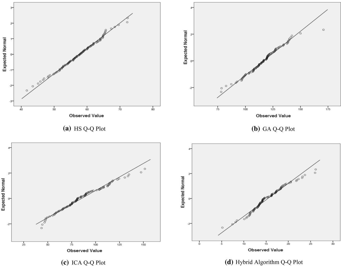
Fig. 16 Q–Q plot for normality test
