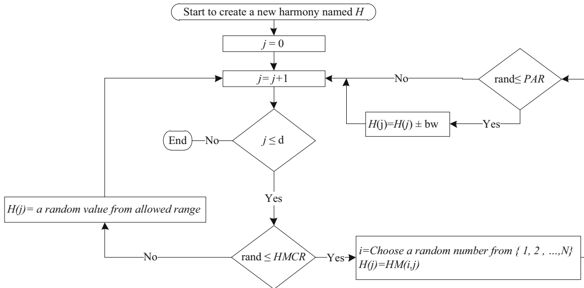
Fig. 3 Process of creation of a new harmony in the HS algorithm
