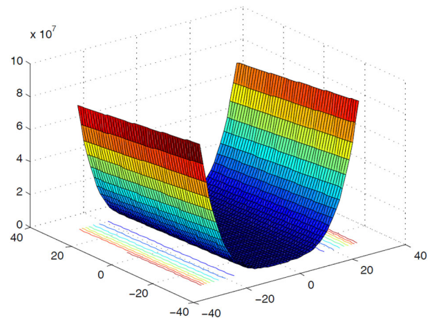
Fig. 9 The Rosenbrock function
