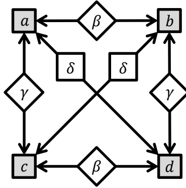
Figure II.6.: If \beta > \gamma > \delta , the efficient team assignment is [(ab)(cd)] . If \beta + \gamma + \delta < -1 , however, the agents unanimously prefer [(ad)(bc)] . Each delegation mechanism would implement [(ad)(bc)] .
