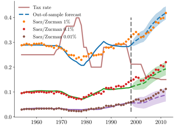
Figure 7: Out-of-sample testing using the time series from years 1954 – 1998 and the 3-dimensional Kalman Filter.
