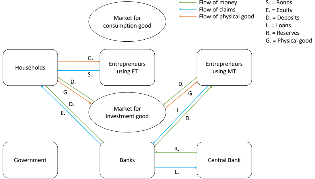
Figure 4: Flows between agents in Period t = 0 .
