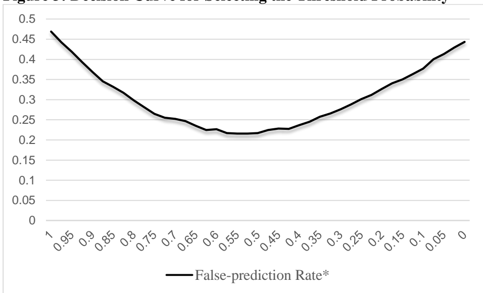
Figure 3: Decision Curve for Selecting the Threshold Probability
