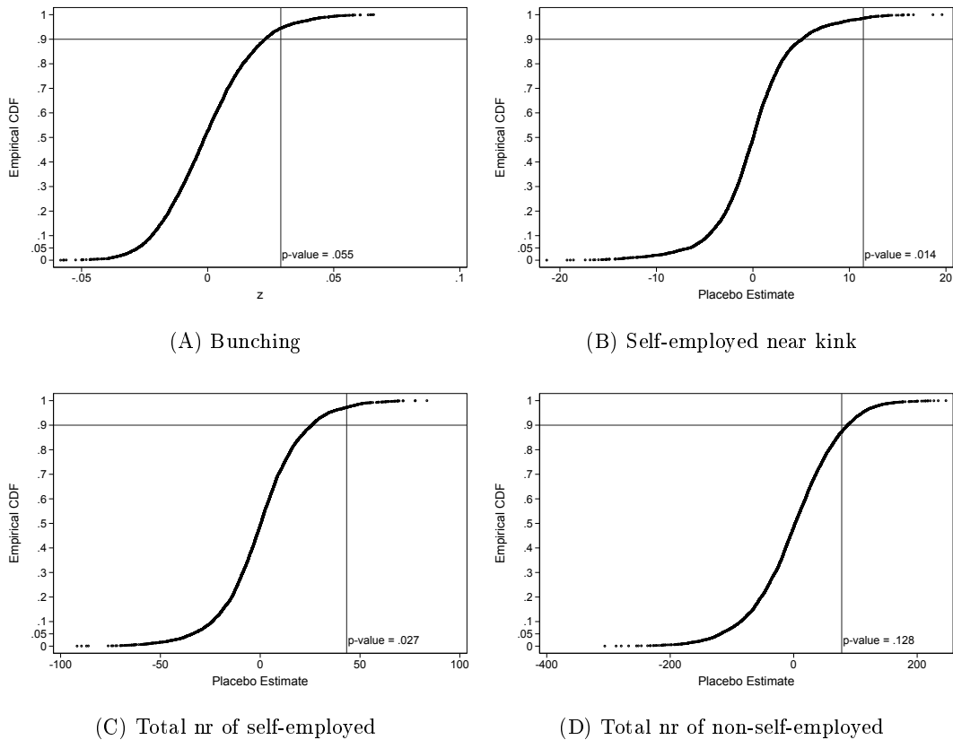
Figure 7: Permutation tests
