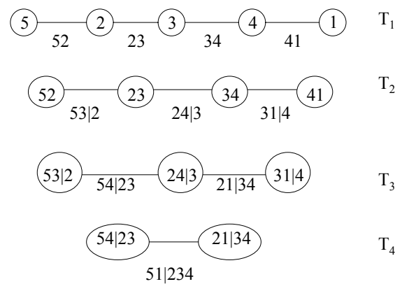
Figure 2. A D-vine with 5 variables, 4 trees and 10 edges. Each edge may be may be associated with a pair-copula.
