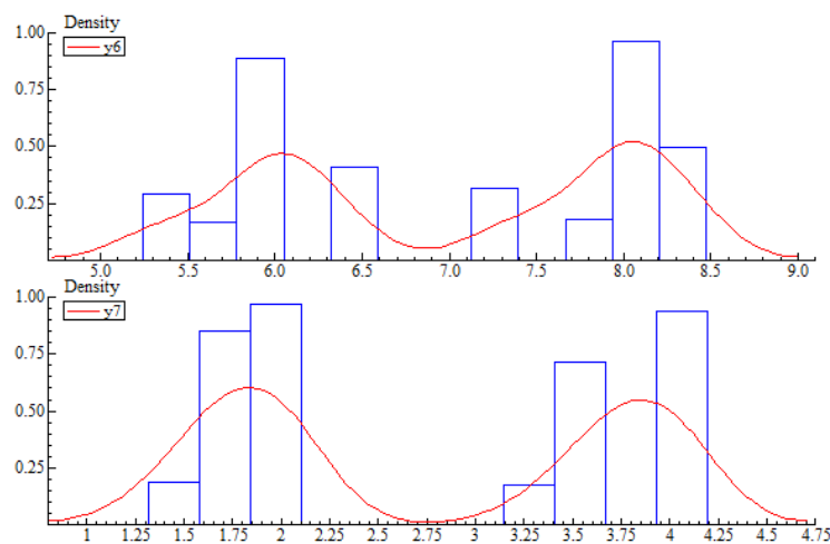
Figure 2. Estimates of the Probability Distributions of y6 and y7.
