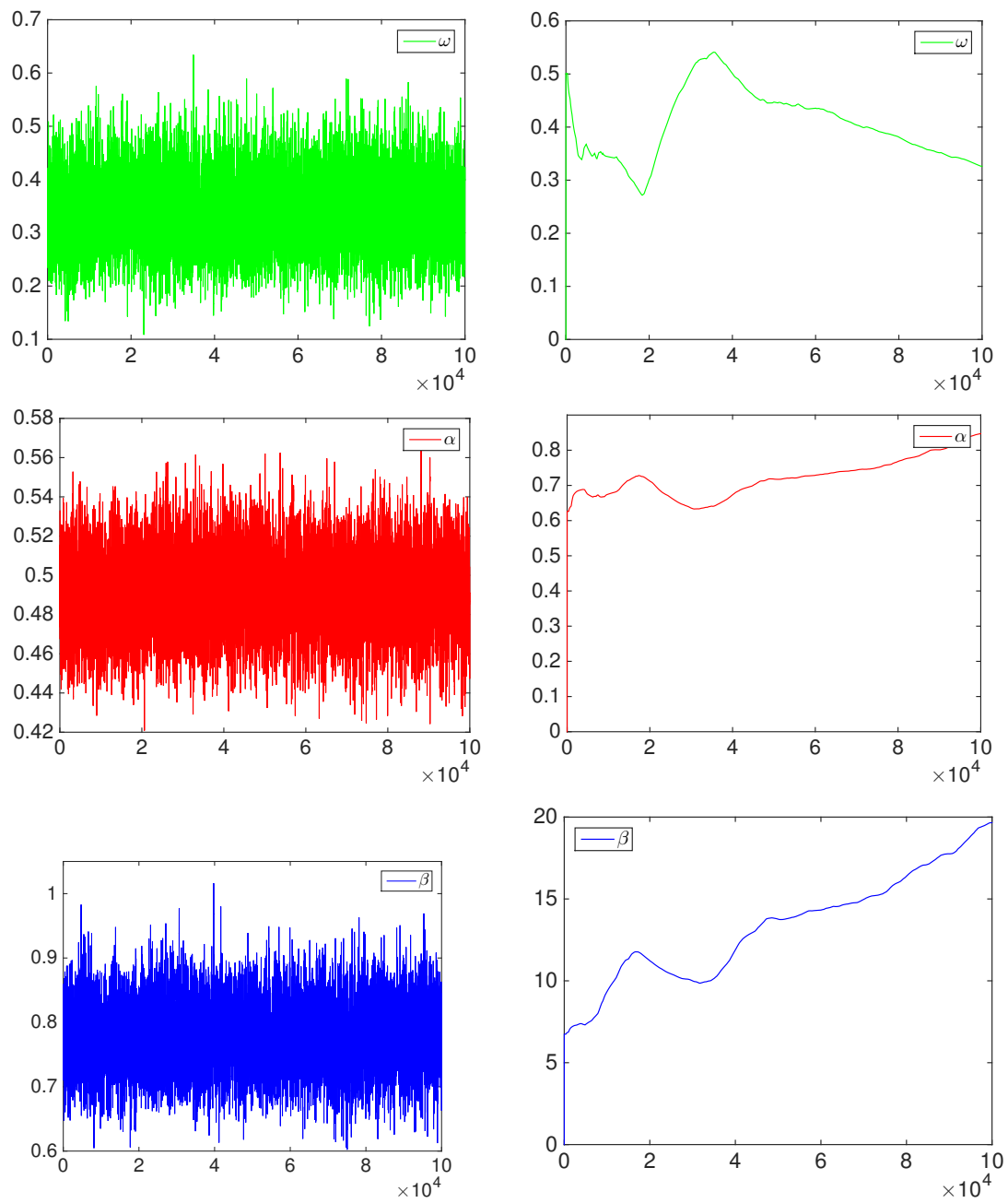
Figure A1. BC1 model ( J = 1 ): 100,000 MCMC samples (left column) and MCMC progressive averages (right column) for the parameters \omega_1 , \alpha_1 and \beta_1 (different rows).
