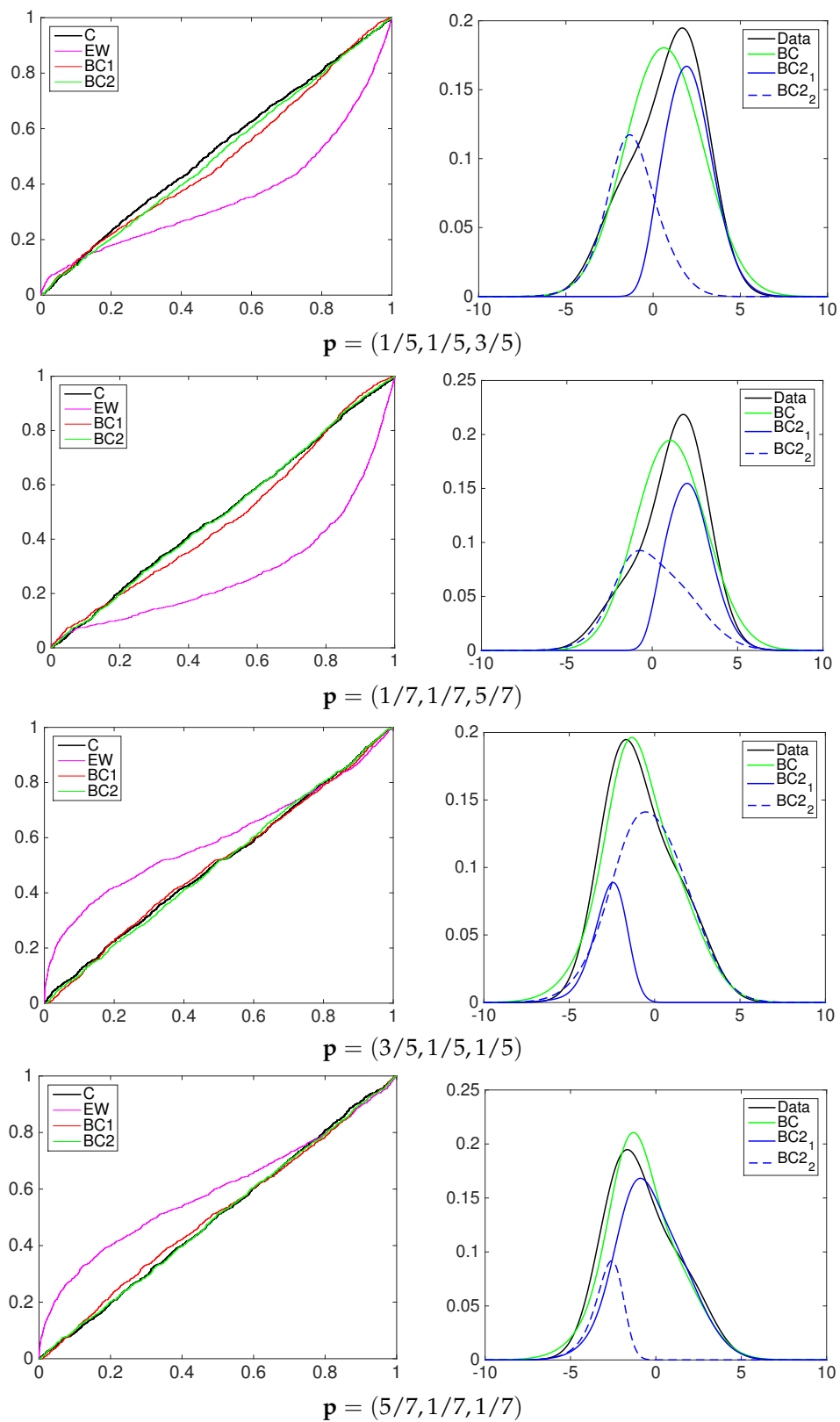
Figure 5. (Left column): PITs' cdf for the linear pool at different values of \mathbf{p} ; (Right column): contribution of calibration components for BC1 (green) and BC2 (blue), where BC2 1 (solid) is the first component of the beta mixture in BC2 and BC2 2 (dashed) the second component.
