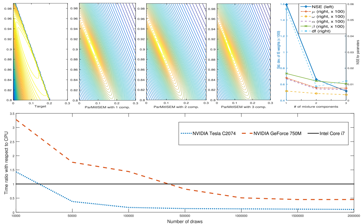
Figure 3. Speed gains and accuracy for the GARCH(1,1) model with Student- t errors. The top-left figure presents the conditional posterior density kernel of (\alpha, \beta) given posterior mean of the other parameters. Second to fourth figures present the evolution of the MitISEM approximation to the posterior kernel for 1–3 mixture components. The top-right panel presents the CoV for the MitISEM approximation and NSE values of each model parameter for different number of components. All MitISEM approximations are based on 100,000 draws. The bottom panel presents the speed comparison for different number of draws, as a GPU/CPU ratio. A value below one indicates the GPU implementation is faster than the CPU implementation.
