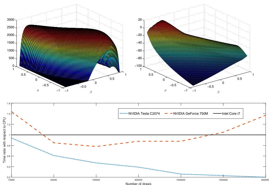
Figure 4. Speed gains and accuracy for the IV model. The top panel in the figure shows the target density apart from an integration constant (left panel) and ParMitISEM candidate (right panel) in natural logarithms. The bottom panel shows the speed comparison for different number of draws, as a GPU/CPU ratio. A value below one indicates that the GPU is faster compared with the CPU.
