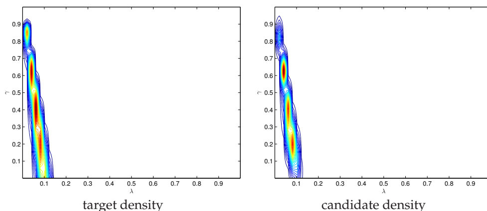
Figure 5. Bayesian inference of the structural NKPC model. The figure shows the posterior density of (\lambda, \gamma) in the structural NKPC model. Remaining model parameters are fixed at their posterior mean.
