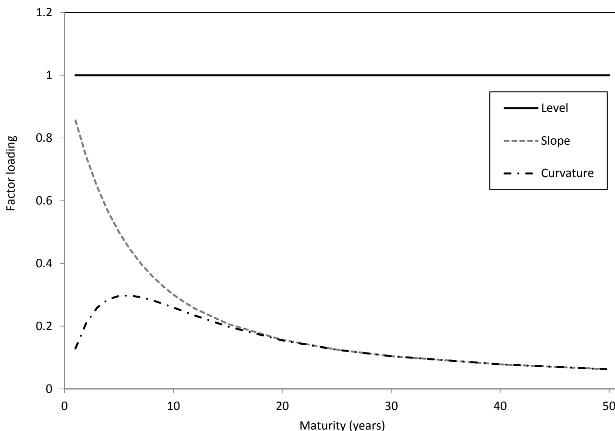
Figure 2. Nelson-Siegel factor loadings ( \lambda = 0.3189 ).
