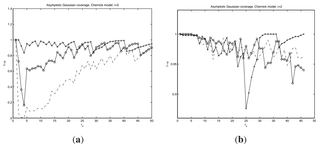
Figure 9. Chernick model with r = 5 in (a) and r = 2 in (b). m = 500 Monte Carlo simulations. +- for n = 200 , o- for n = 500 and -- for n = 1000 . \hat{u}_n = M_{t+1:k_n} and \hat{v}_n = X_{t+1:n} with t = \lceil 0.005k_n \rceil , where \lceil \cdot \rceil rounds to the next integer. r_n = [1, 50] , k_n = n/r_n . \alpha = 0.05 .
