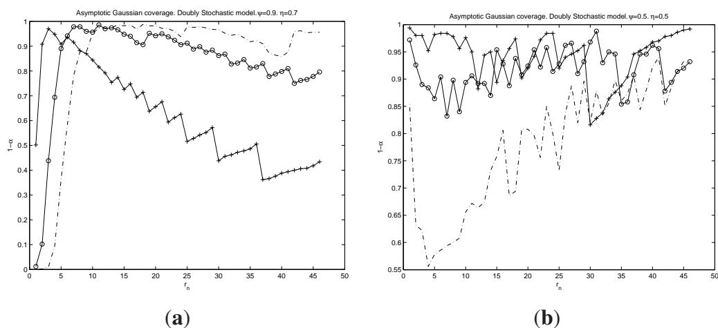
Figure 10. Doubly-stochastic model with \psi = 0.9 and \eta = 0.7 and \psi\eta = 0.5 in (a) and \eta = 0.5 in (b). m = 500 Monte Carlo simulations. +- for n = 200 , o- for n = 500 and -- for n = 1000 . \hat{u}_n = M_{t+1:k_n} and \hat{v}_n = X_{t+1:n} with t = \lceil 0.005k_n \rceil , where \lceil \cdot \rceil rounds to the next integer. r_n = [1, 50] , k_n = n/r_n . \alpha = 0.05 .
