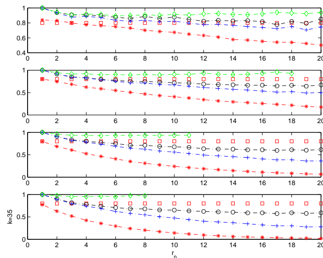
Figure 1. Chernick model with r = 5 . \theta = 0.8 . Sample mean for different estimators of \theta . m = 100 Monte Carlo simulations. \hat{u}_n = M_{t+1:k_n} , and \hat{v}_n = X_{t+1:n} with t = 1, 3, 5, 7 ; n = 200 . r_n \in [1, 20] . \theta plotted with, \tilde{\theta}_n^f with -o , \hat{\theta}_n^{(1)} with -\diamond , \hat{\theta}_n^{(2)} with -+ , and \bar{\theta}_n with the -* line.
