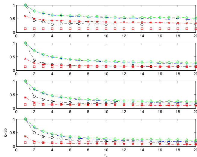
Figure 3. Doubly-stochastic model with \psi = 0.9 and \eta = 0.7 . \theta = 0.137 . Sample mean for different estimators of \theta . m = 100 Monte Carlo simulations. \hat{u}_n = M_{t+1:k_n} , and \hat{v}_n = X_{t+1:n} , with t = 1, 3, 5, 7 ; n = 200 . r_n \in [1, 20] . \theta plotted with -o , \tilde{\theta}_n^f with -o , \hat{\theta}_n^{(1)} with -\diamond , \hat{\theta}_n^{(2)} with -+ , and \bar{\theta}_n with the -* line.
