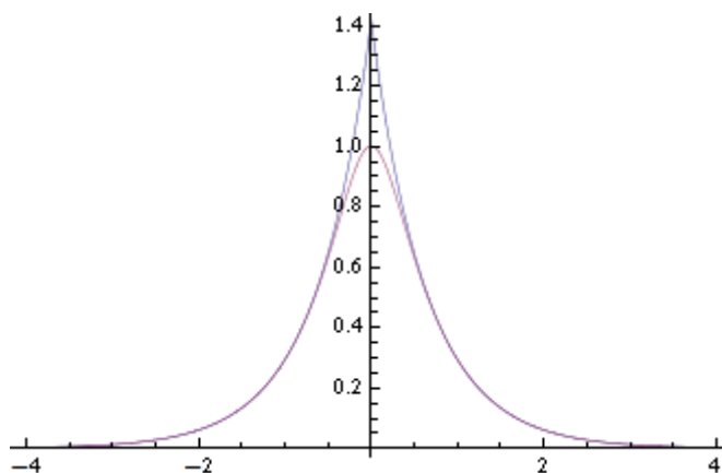
Figure 2. Modulus function of the characteristic function of logarithmic chi-square distribution and its approximation: the higher peak curve is the approximating function \sqrt{2}e^{-\frac{1}{2}\pi|t|} .
