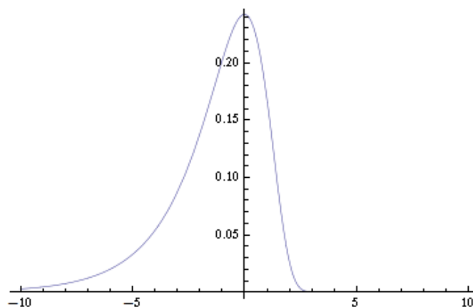
Figure 1. Density function of the logarithmic chi-square distribution.
