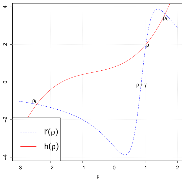
Figure 2. Intersection points of h(\rho) and l'(\rho) when T = 5 , \underline{\rho} = 1 , \sigma^2 = 1 , \sigma_f^2 = 1 , \sigma_{y_0}^2 = 0.1 , E(f_i) = E(y_{i,0}) = E(f_i y_{i,0}) = 0 and there are no exogenous regressors.
