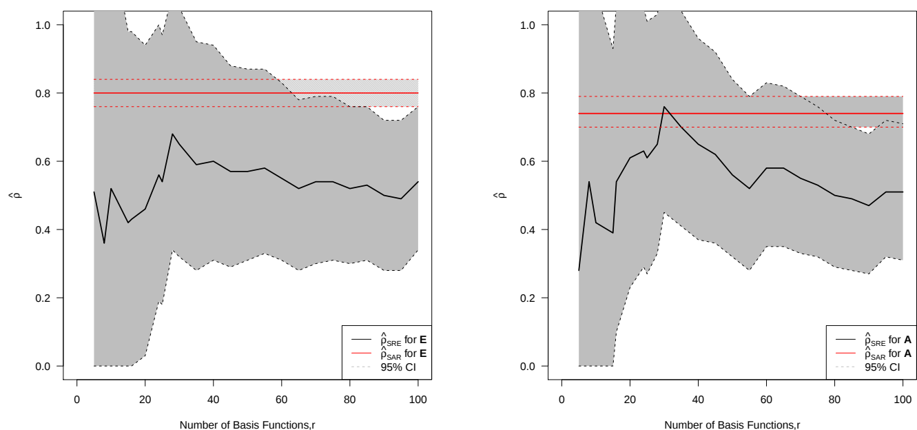
Figure 4. SAR-calibrated spatial random effects (SRE) model restricted (or residual) maximum likelihood (REML) estimates for \hat{\rho} and \hat{\sigma}_v^2 for SW Sydney as a function of r for \mathbf{E} (left-hand panel) and for \mathbf{A} (right-hand panel); the SAR model estimate \hat{\rho}_{SAR} and 95% profile log-likelihood confidence intervals (CI) for \rho are included for comparison (36).
