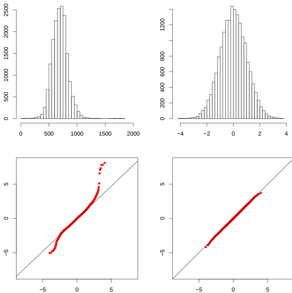
Figure 2. Histogram and Q-Q plot of \mathbf{Z} for 16,850 SA1 areas (left panels). Histogram and Q-Q plot of standardised values (41) for the same SA1 areas (right panels).
