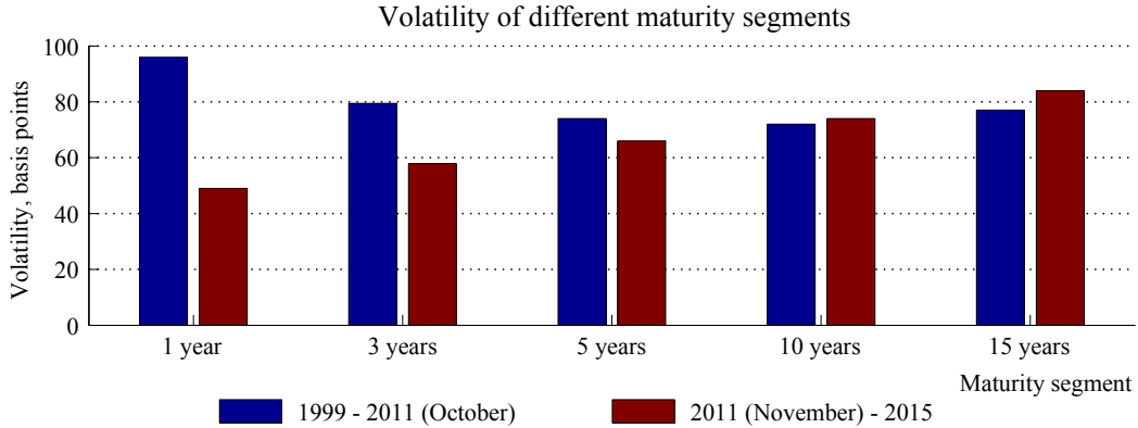
Figure 1: Volatility of Danish government bond yields with different maturities, before and during low-rate period. The volatility is calculated as the (annualised) standard deviation of daily zero-coupon bond yield changes.
