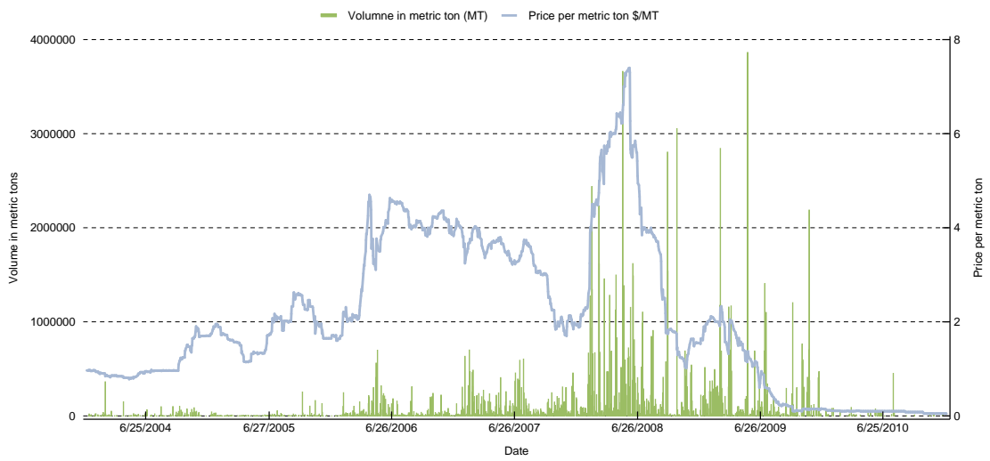
Figure A1: CCX Daily Average Volume (metric ton) and settlement price
