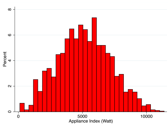
Figure 4: Histogram of Appliance Index
