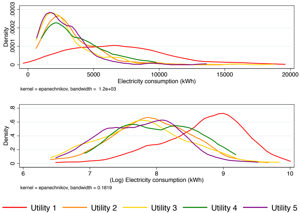
Figure 2: Kernel Density Plot for 2011
