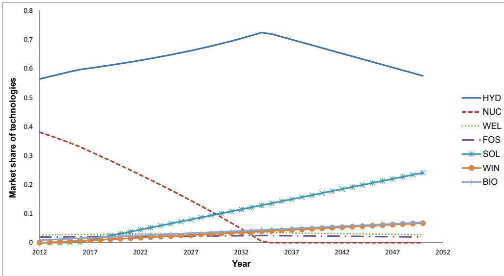
Figure 4: Share of generation technologies in PO-CC
