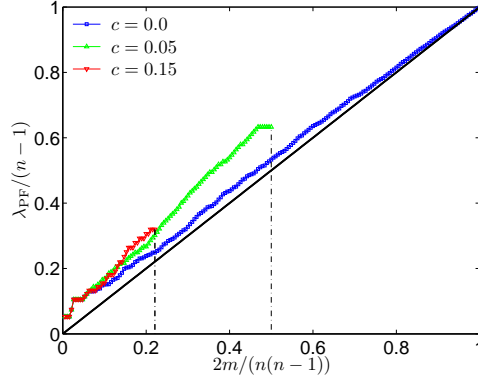
Fig. 5. Largest real eigenvalue \lambda_{\text{PF}} of a network of n = 20 firms as a function of the number m of links, along three specific improving paths for costs c = 0.0 , c = 0.05 , c = 0.15 and severance cost parameter \alpha = 0 . The number of links m and the largest real eigenvalue \lambda_{\text{PF}} are normalized to their maximum values (attained by the complete graph). The improving path for cost c = 0.15 reaches 22% of the density of a complete graph before it arrives at a stable network while the improving path for cost c = 0.05 reaches already 50% of the maximum density. Obviously the improving path for c = 0 reaches the complete graph.
