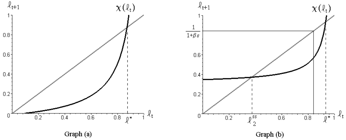
Figure 1: Examples of stationary solutions for work time in the decentralized equilibrium. Graph (a): when b_1 < 0 there exists a unique equilibrium ( \alpha = 0.3 , \beta = 0.65 , \varepsilon = 0.6 ). Graph (b): when b_1 > 0 there exists a second solution \ell_2^{ss} < \ell_1^{ss} but it violates optimality conditions ( \alpha = 0.3 , \beta = 0.65 , \varepsilon = 0.3 ). The other solution thus represents the equilibrium.
