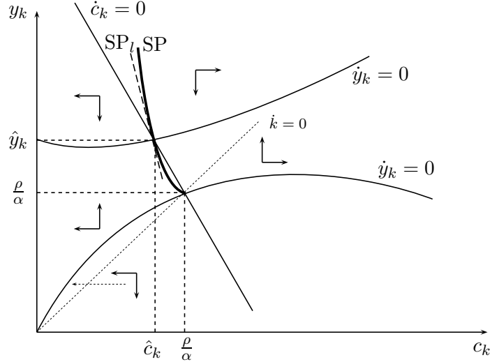
Figure 4: Transitional dynamics for \sigma < \alpha (Scenario 2)
