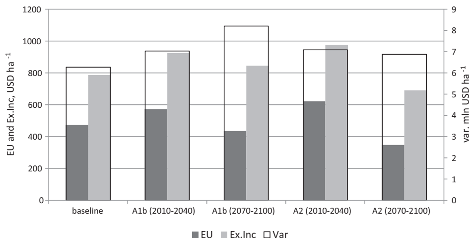
Fig. 4. Expected utility, expected income and variance change in the representative farm under different scenarios (semiarid, Uzbekistan).
