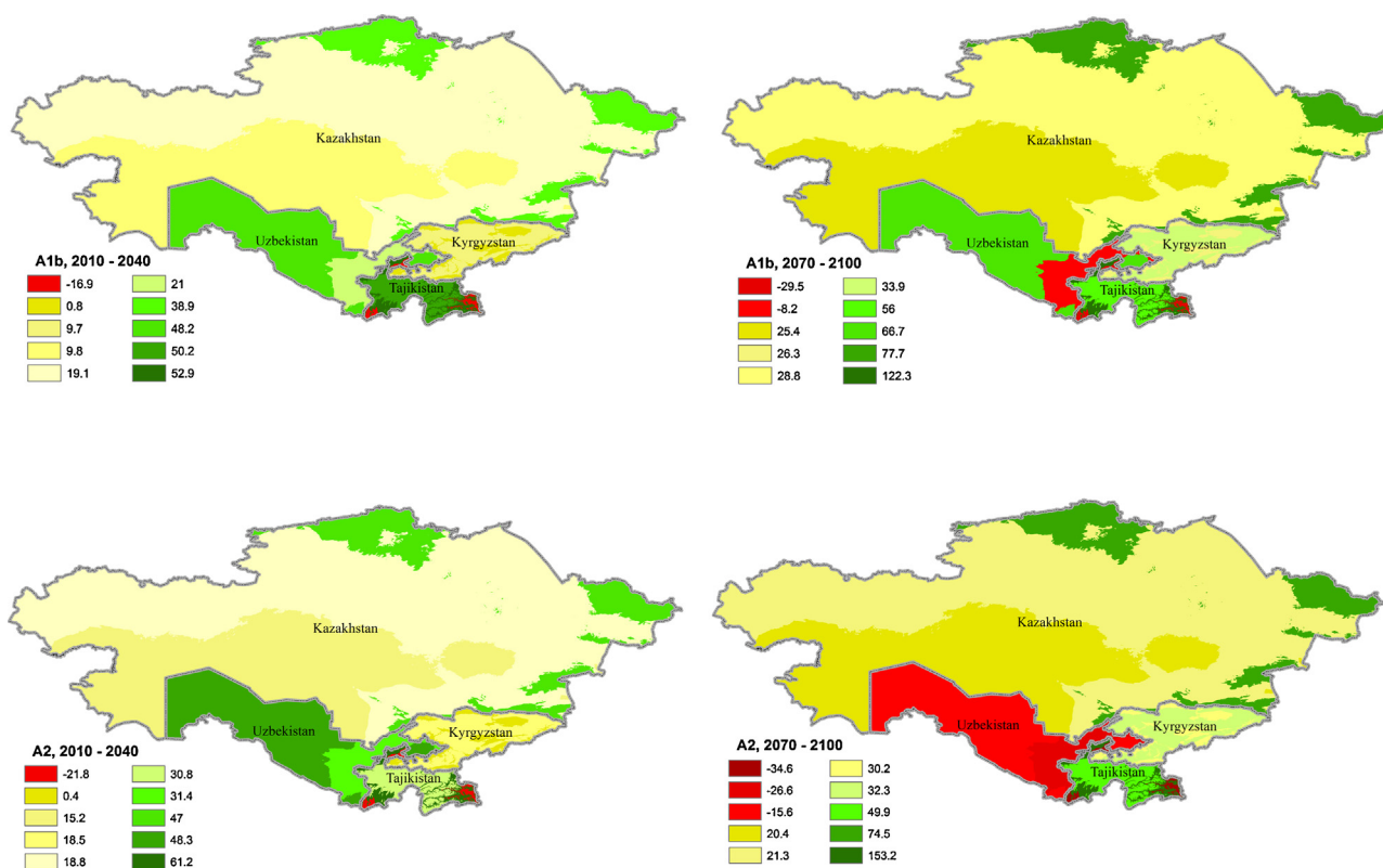
Fig. 6. Percentage changes of expected utility to the baseline scenario. (For interpretation of the references to colour in this figure legend, the reader is referred to the web version of this article.)
