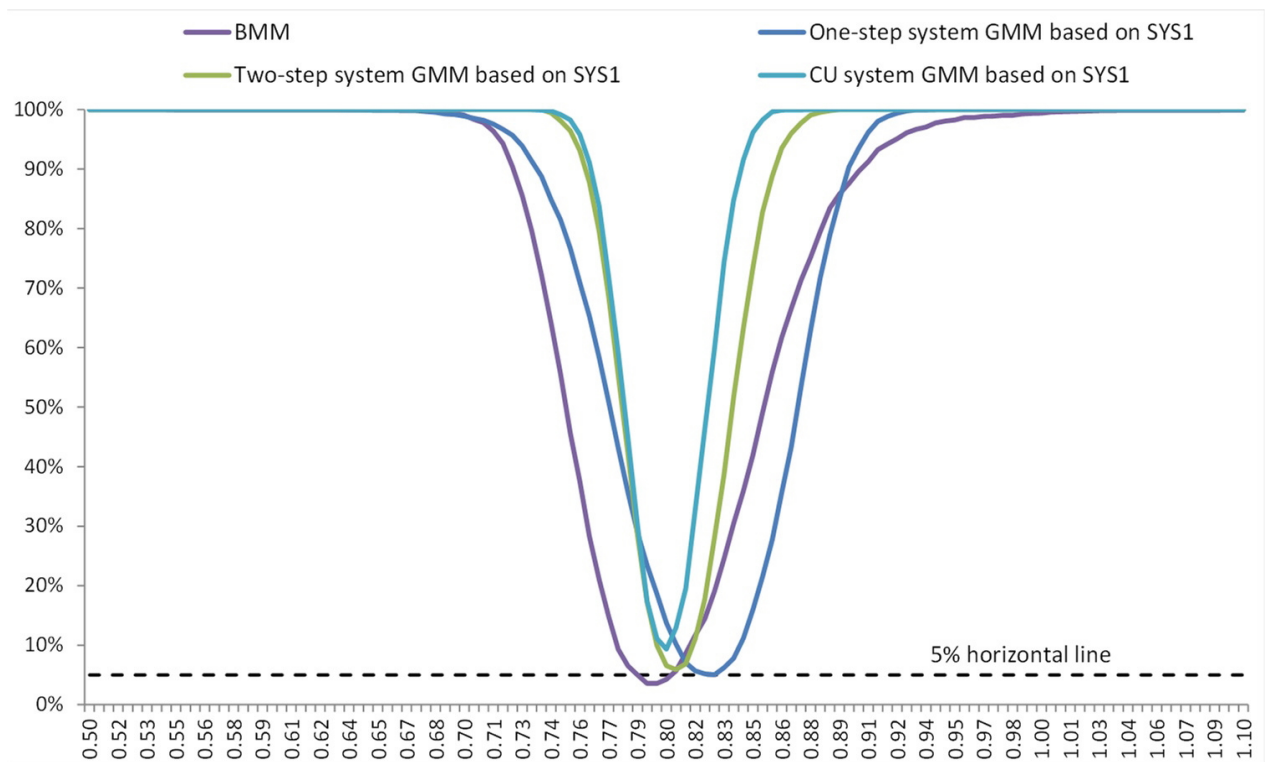
Figure S3: Rejection frequency of the tests based on the BMM and the system GMM estimators based on SYS1 moment conditions in Experiment 1 ( \phi = 0.8 , \mu_v = 0 ), for sample size n = 1000 and T = 10 . S5
