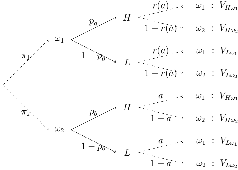
Figure 2: Decomposition with two outcomes (2)
