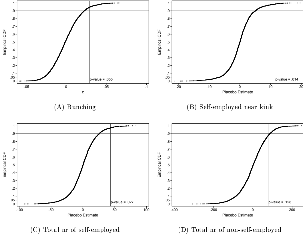
Figure 7: Permutation tests
