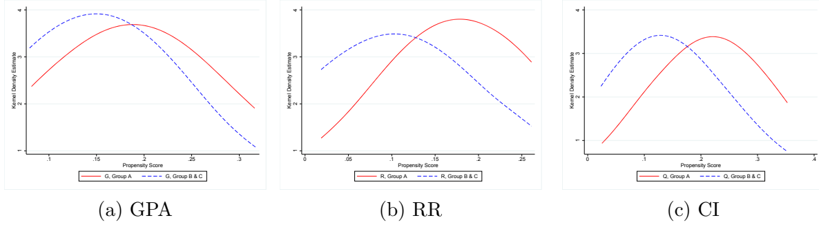
Figure A.3: Propensity score distribution of Group A vs. B & C of the IQR
