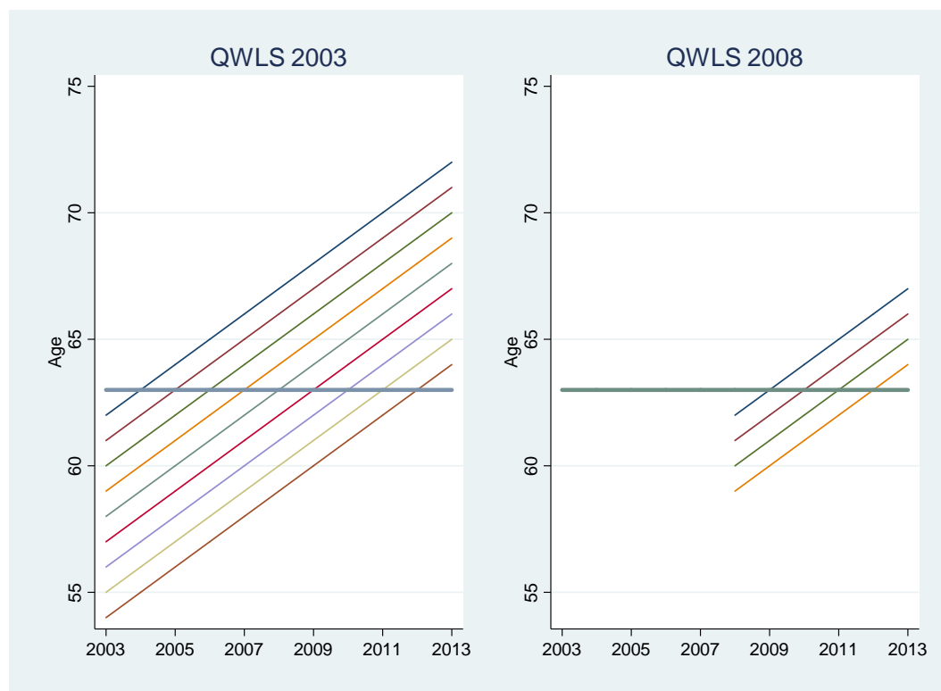
Figure 1. Lexis diagram of birth cohorts included in the estimations.
