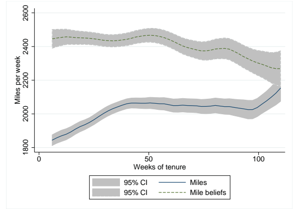
(b) Medians
