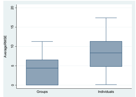
Figure 4: Average RMSE across treatments in winners instances
