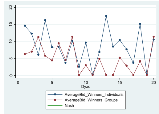
Figure 2: dyads' bid distributions averaged over time for winners
