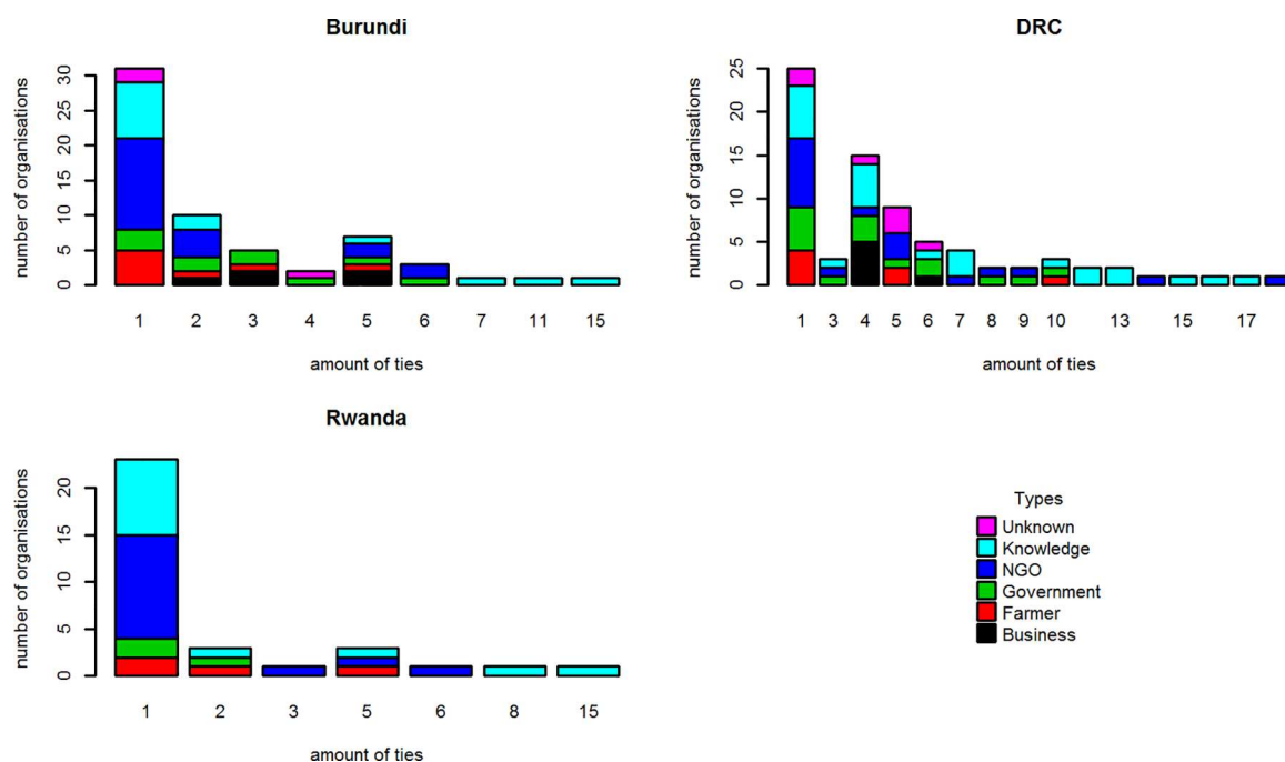
Fig 2. Distribution of knowledge degrees among different types of organisations.
