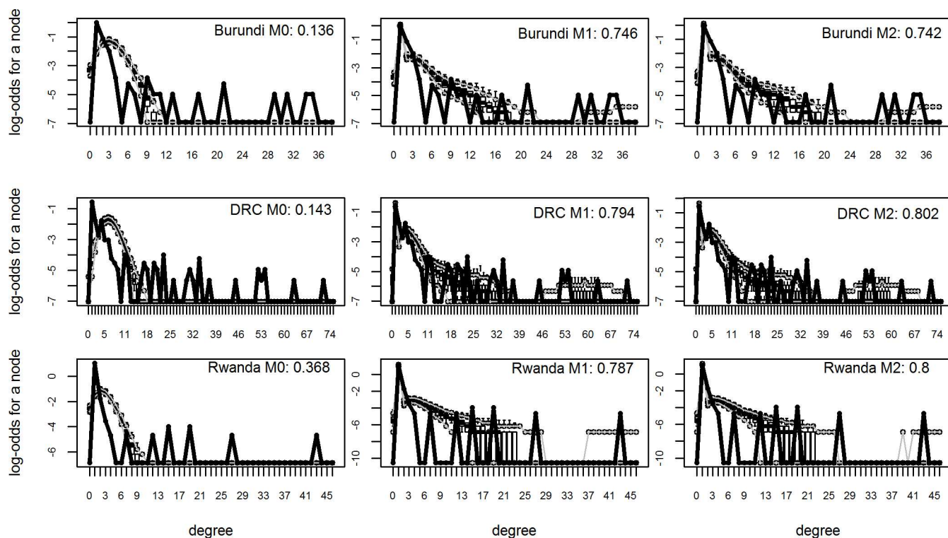
Fig 4. Goodness of fit over the degree distribution for different model forms.
