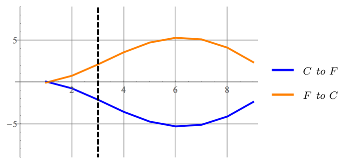
Figure 15.b: Stackelberg Game without PFTA ( m^* = 3 )
