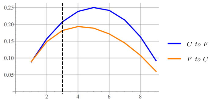
Figure 14.b: Stackelberg Game without PFTA ( m^* = 3 )
