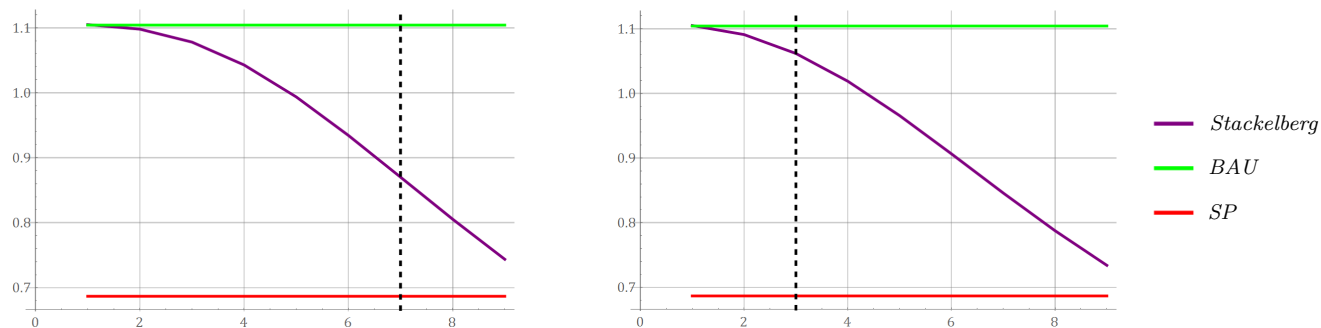
Figure 2.a: Stackelberg Game with PFTA ( m^* = 7 )
