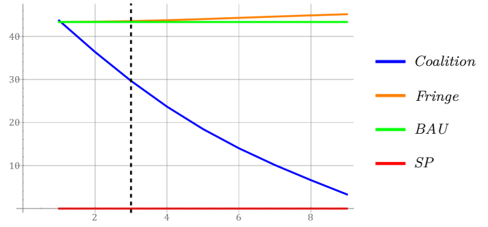
Figure 6.b: Stackelberg Game without PFTA ( m^* = 3 )
