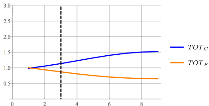
Figure 8.b: Stackelberg Game without PFTA ( m^* = 3 )
