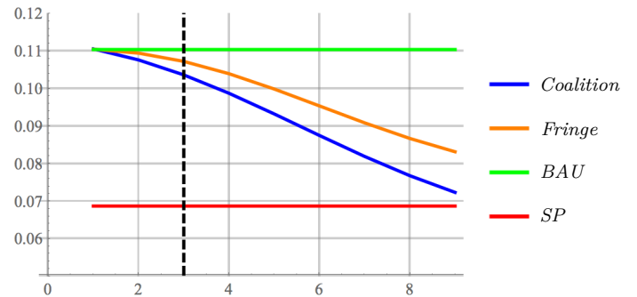
Figure 10.b: Stackelberg Game without PFTA ( m^* = 3 )
