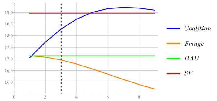
Figure 12.b: Stackelberg Game without PFTA ( m^* = 3 )
