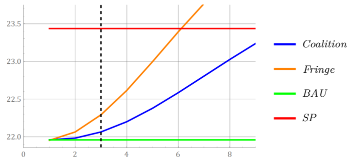
Figure 5.b: Stackelberg Game without PFTA ( m^* = 3 )
