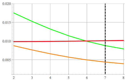
Figure 7.a: Stackelberg Game with PFTA ( m^* = 7 )
