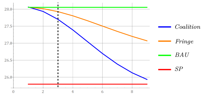
Figure 13.b: Stackelberg Game without PFTA ( m^* = 3 )
