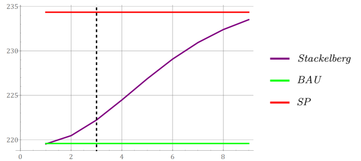
Figure 4.b: Stackelberg Game without PFTA ( m^* = 3 )
